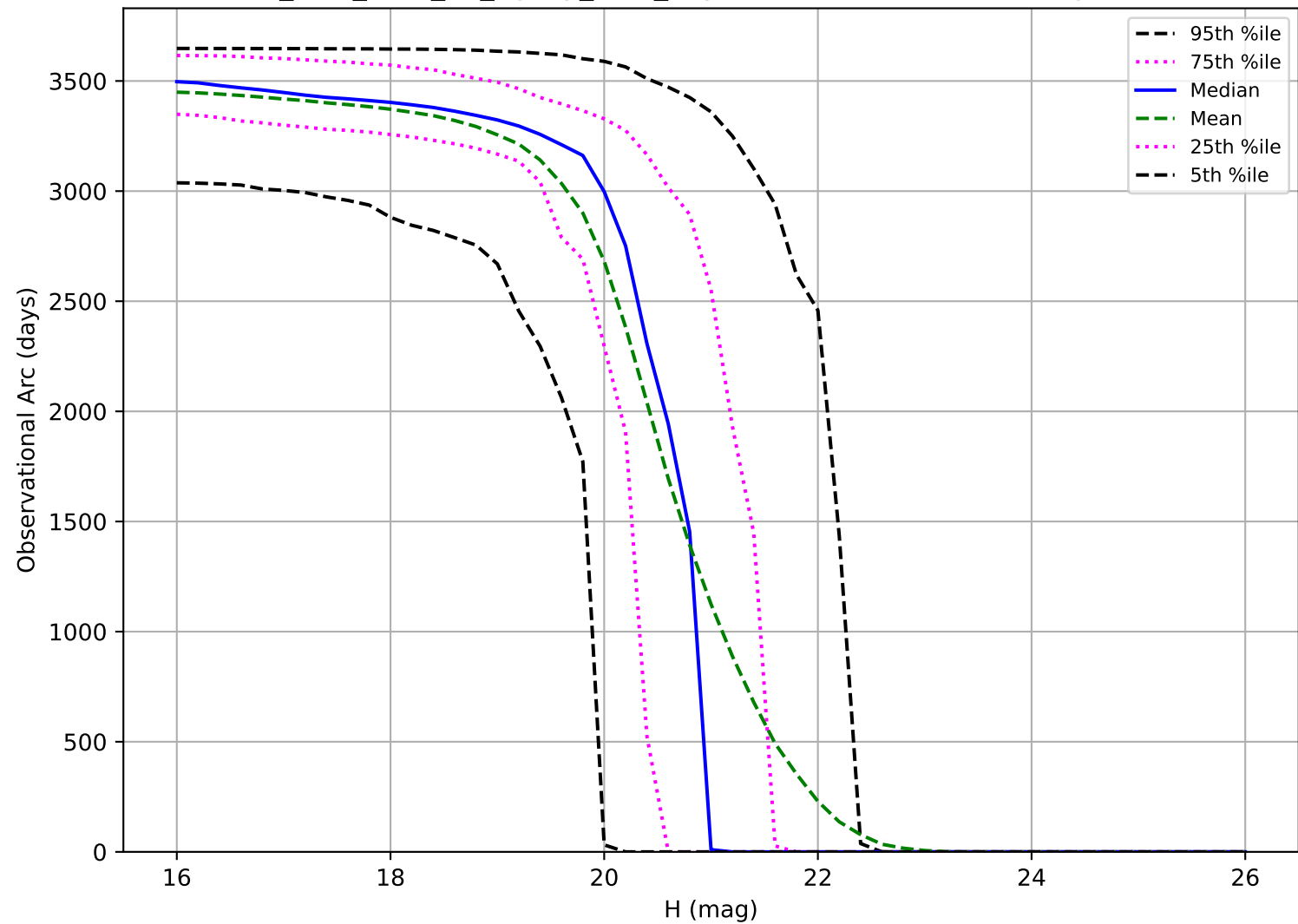
too_elab_r256_d3_ugrizy_v3.4_10yrs: Observational Arc Length MBA
