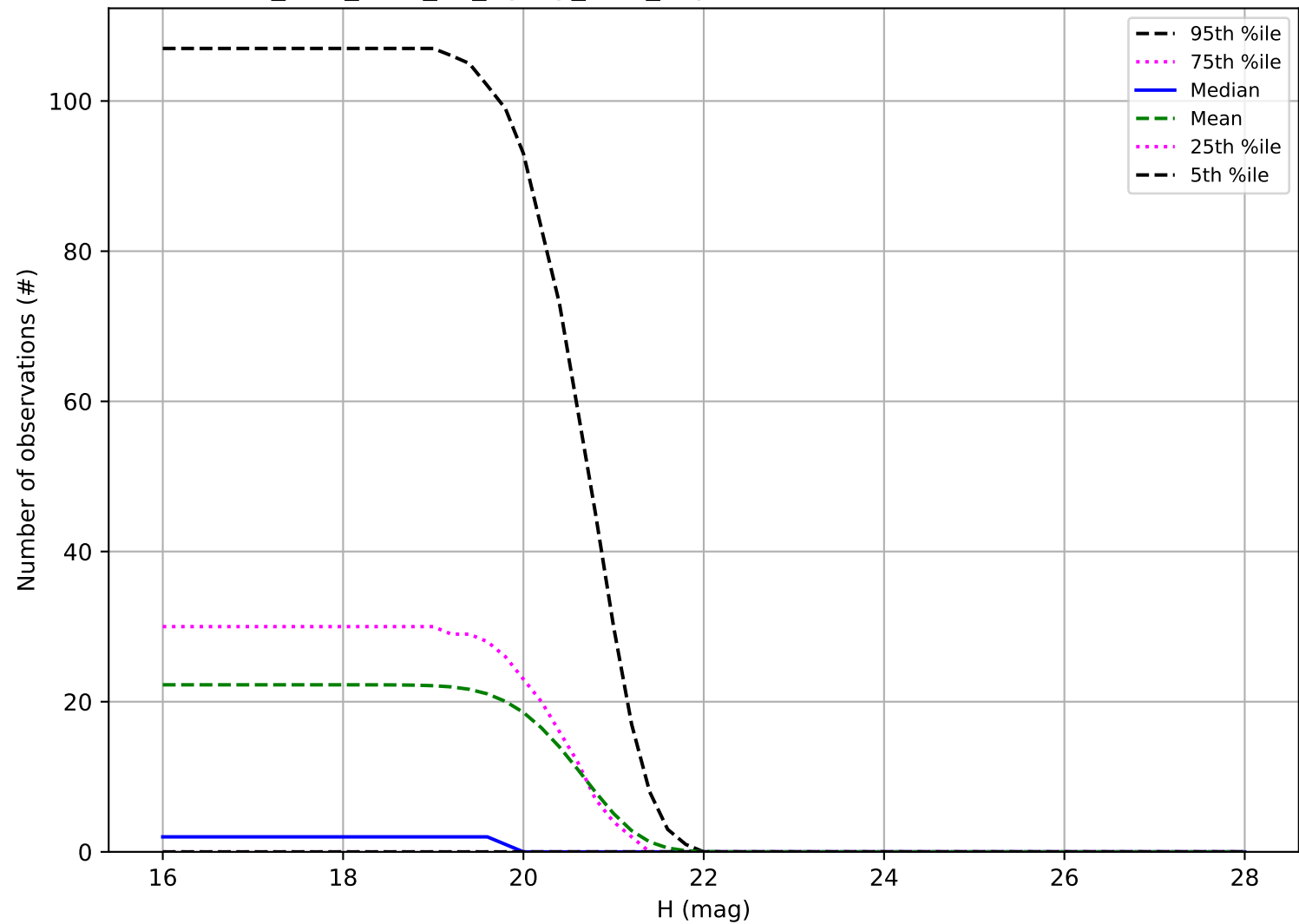
too_elab_r256_d3_ugrizy_v3.4_10yrs: Number of observations Vatira
