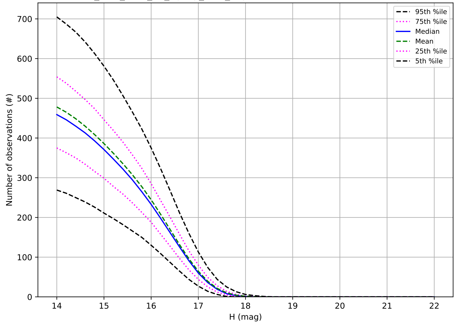
too_elab_r256_d3_ugrizy_v3.4_10yrs: Number of observations Trojan
