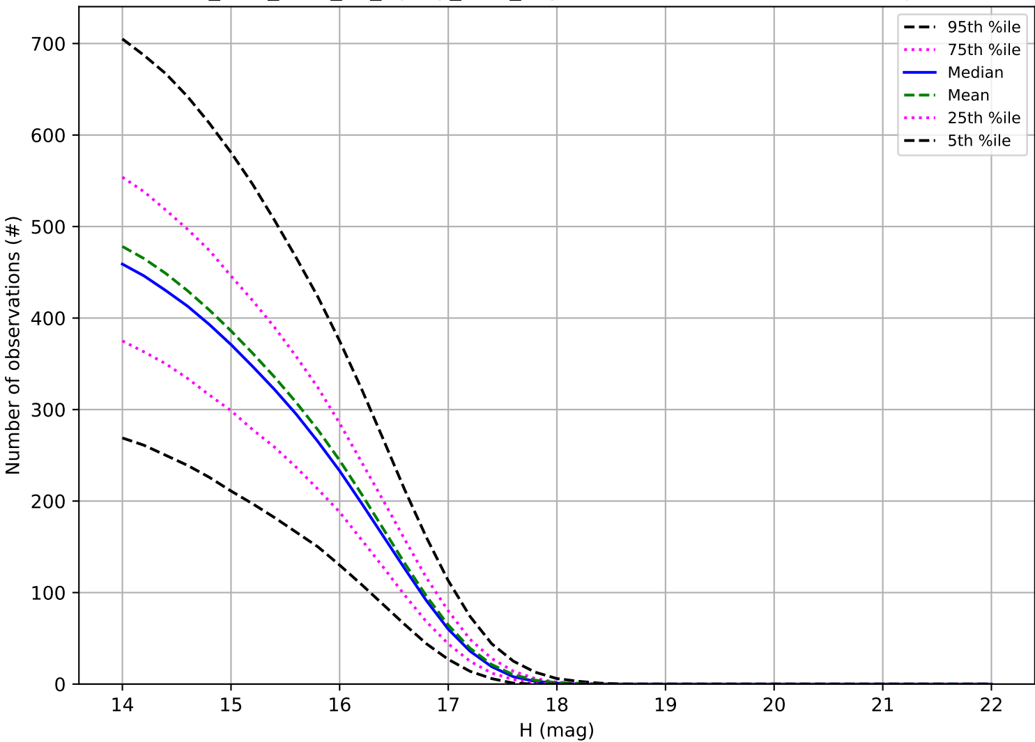
too_elab_r256_d3_ugrizy_v3.4_10yrs: Number of observations Trojan
