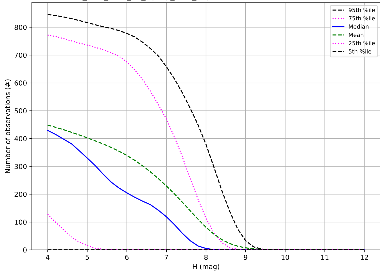
too_elab_r256_d3_ugrizy_v3.4_10yrs: Number of observations TNO
