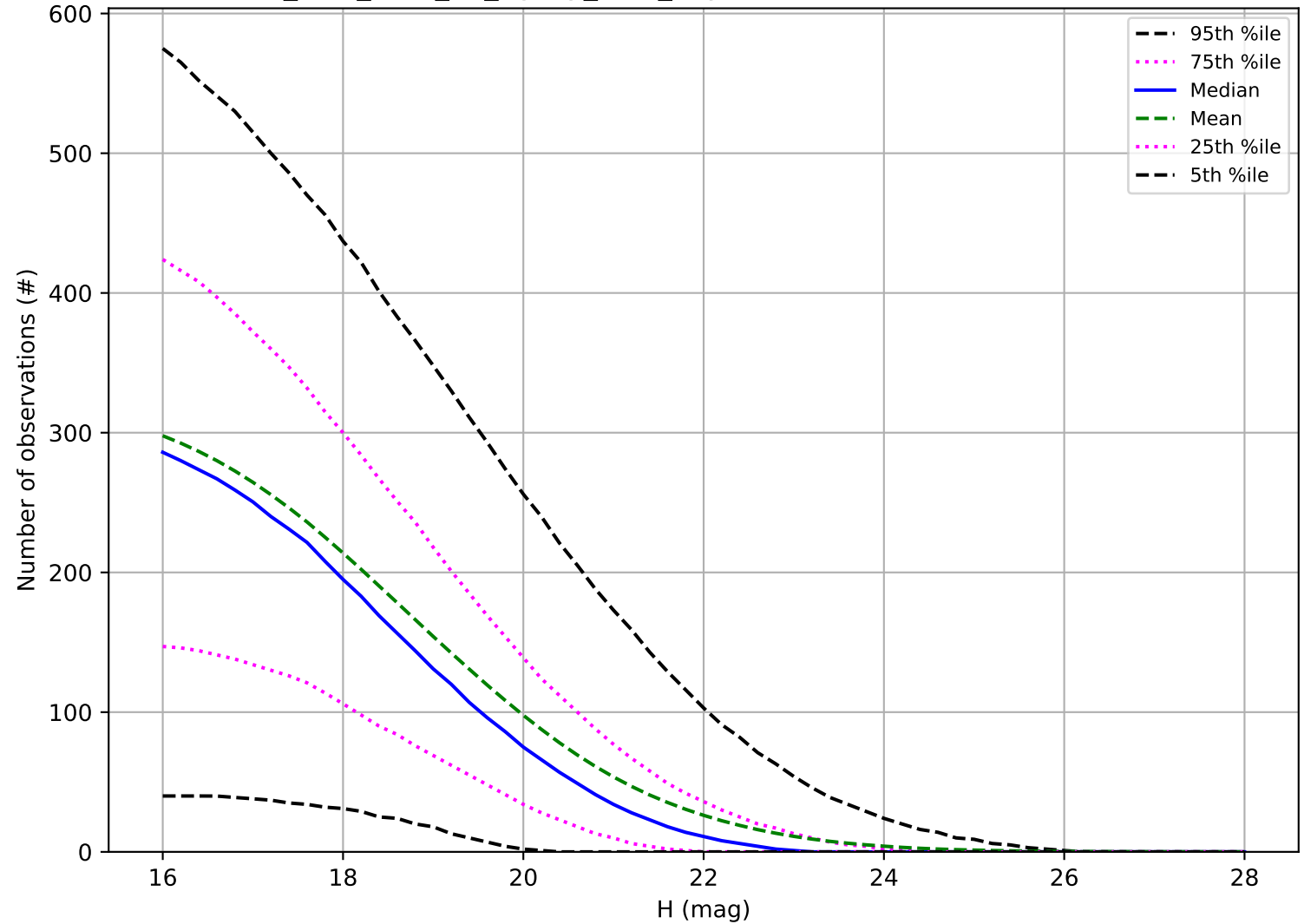
too_elab_r256_d3_ugrizy_v3.4_10yrs: Number of observations PHA
