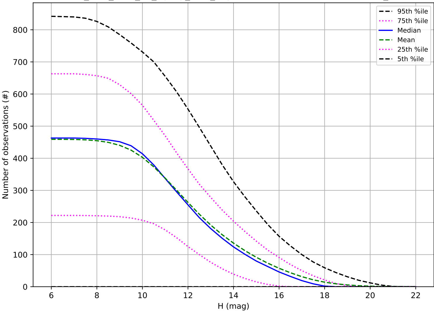
too_elab_r256_d3_ugrizy_v3.4_10yrs: Number of observations OCC_r5
