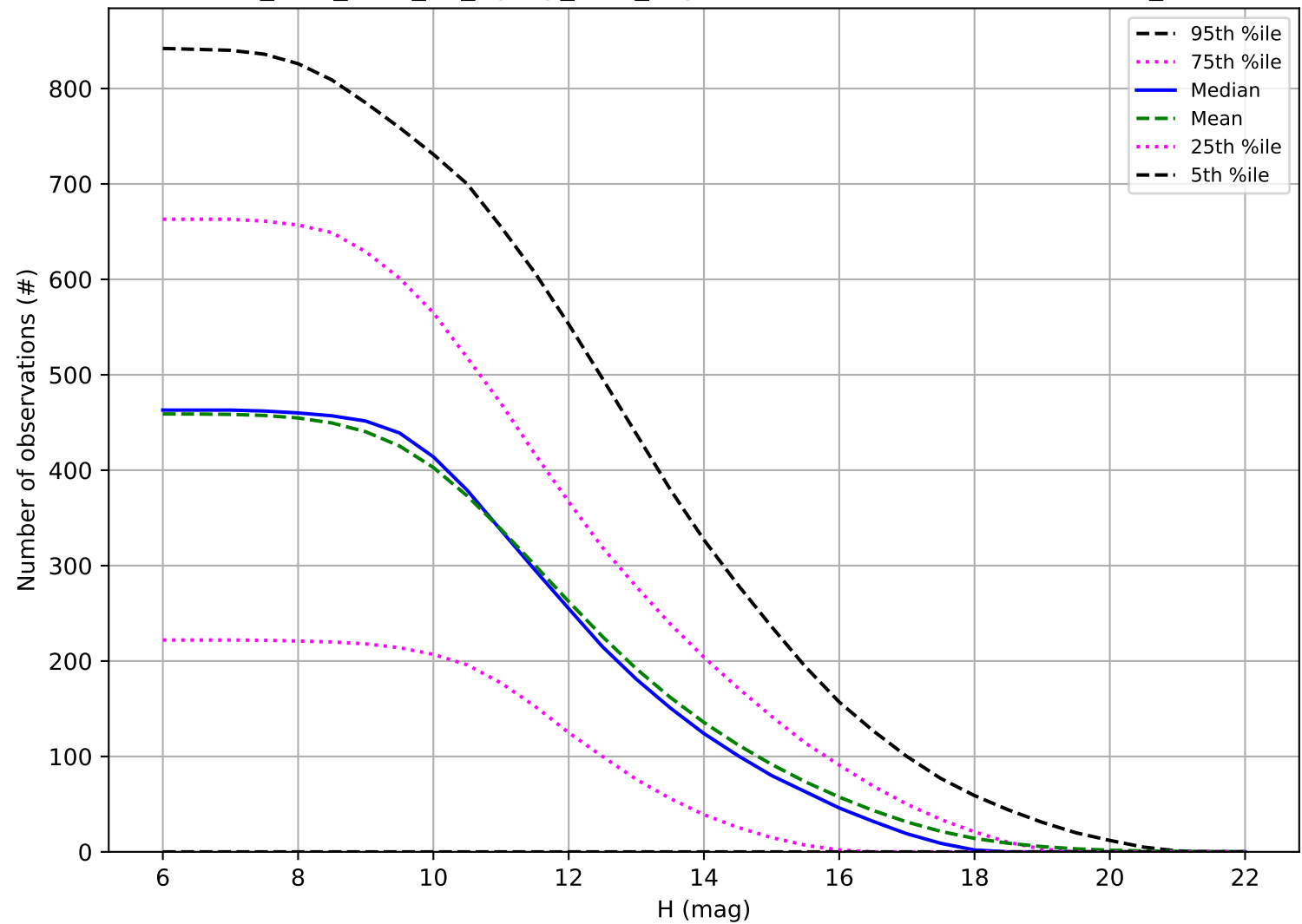
too_elab_r256_d3_ugrizy_v3.4_10yrs: Number of observations OCC_r5
