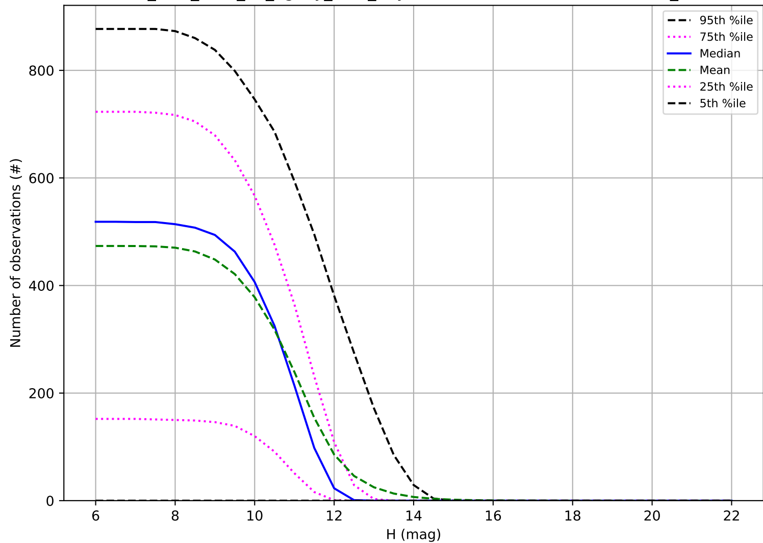
too_elab_r256_d3_ugrizy_v3.4_10yrs: Number of observations OCC_r20
