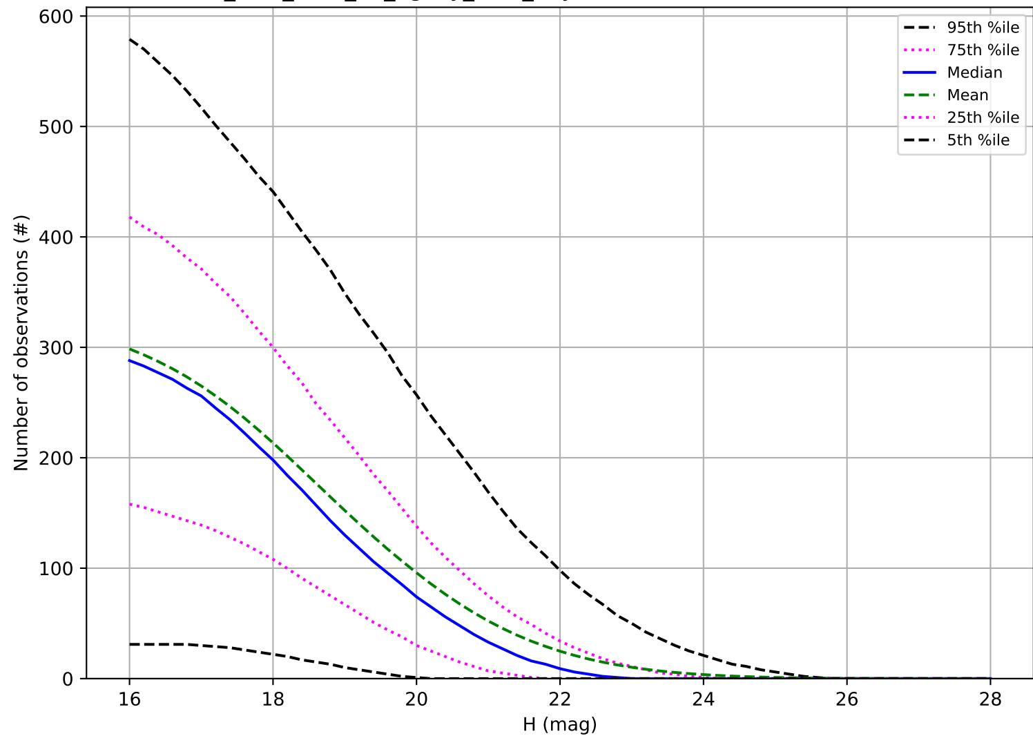
too_elab_r256_d3_ugrizy_v3.4_10yrs: Number of observations NEO
