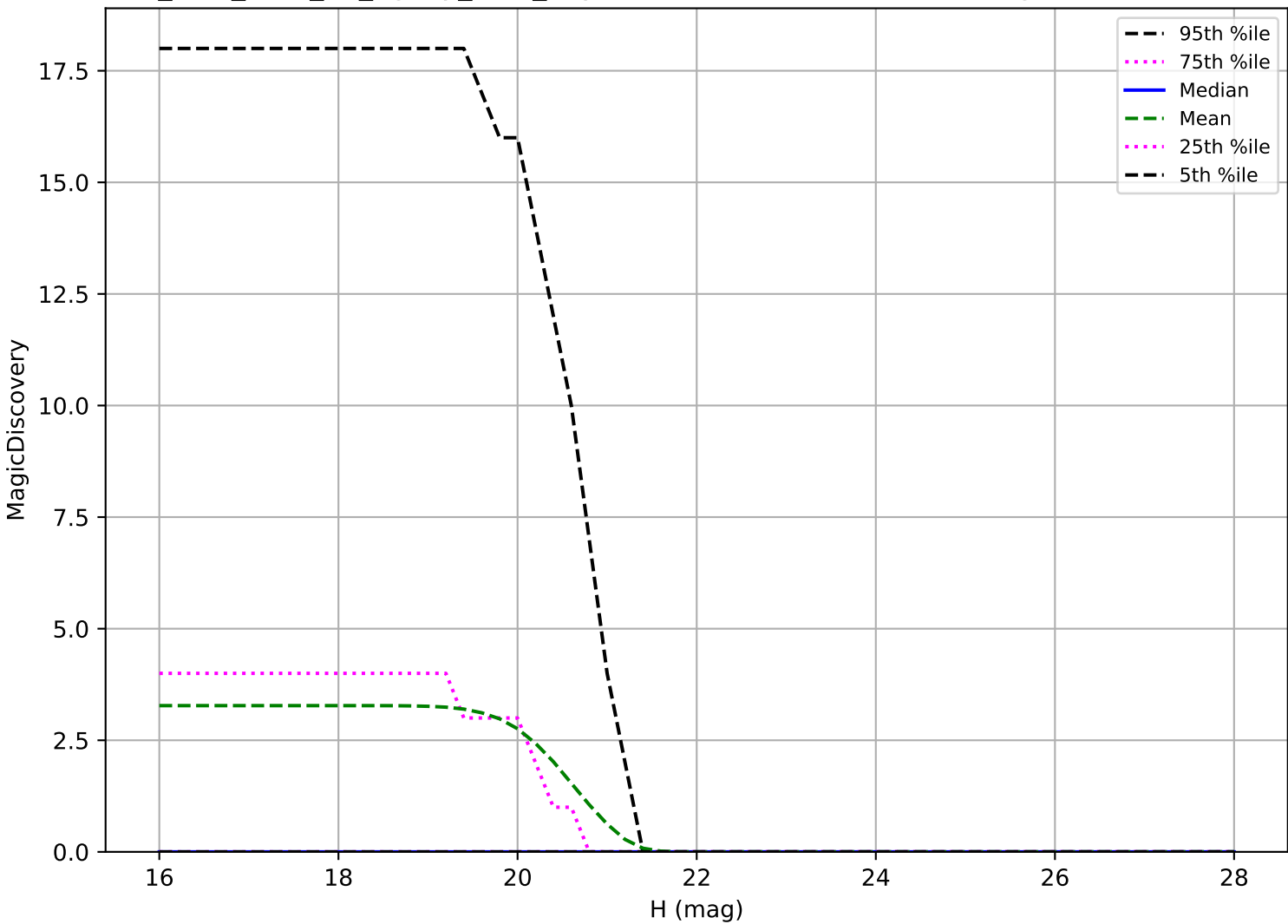
too_elab_r256_d3_ugrizy_v3.4_10yrs: Vatira 6 detections in 60 nights detection loss
