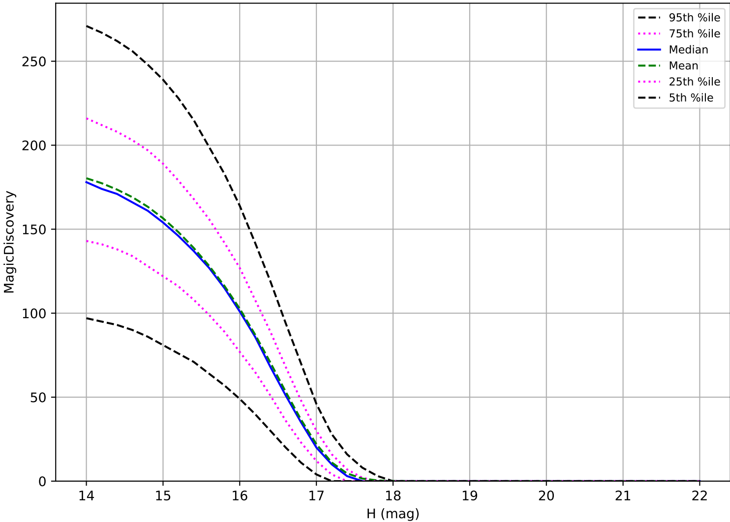
too_elab_r256_d3_ugrizy_v3.4_10yrs: Trojan 6 detections in 60 nights detection loss
