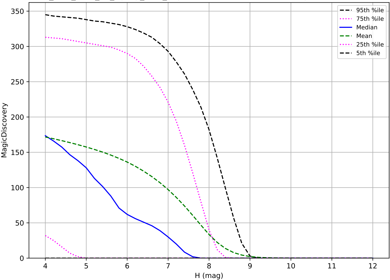
too_elab_r256_d3_ugrizy_v3.4_10yrs: TNO 6 detections in 60 nights detection loss
