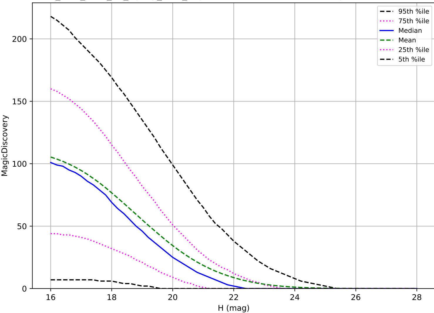
too_elab_r256_d3_ugrizy_v3.4_10yrs: PHA 6 detections in 60 nights detection loss
