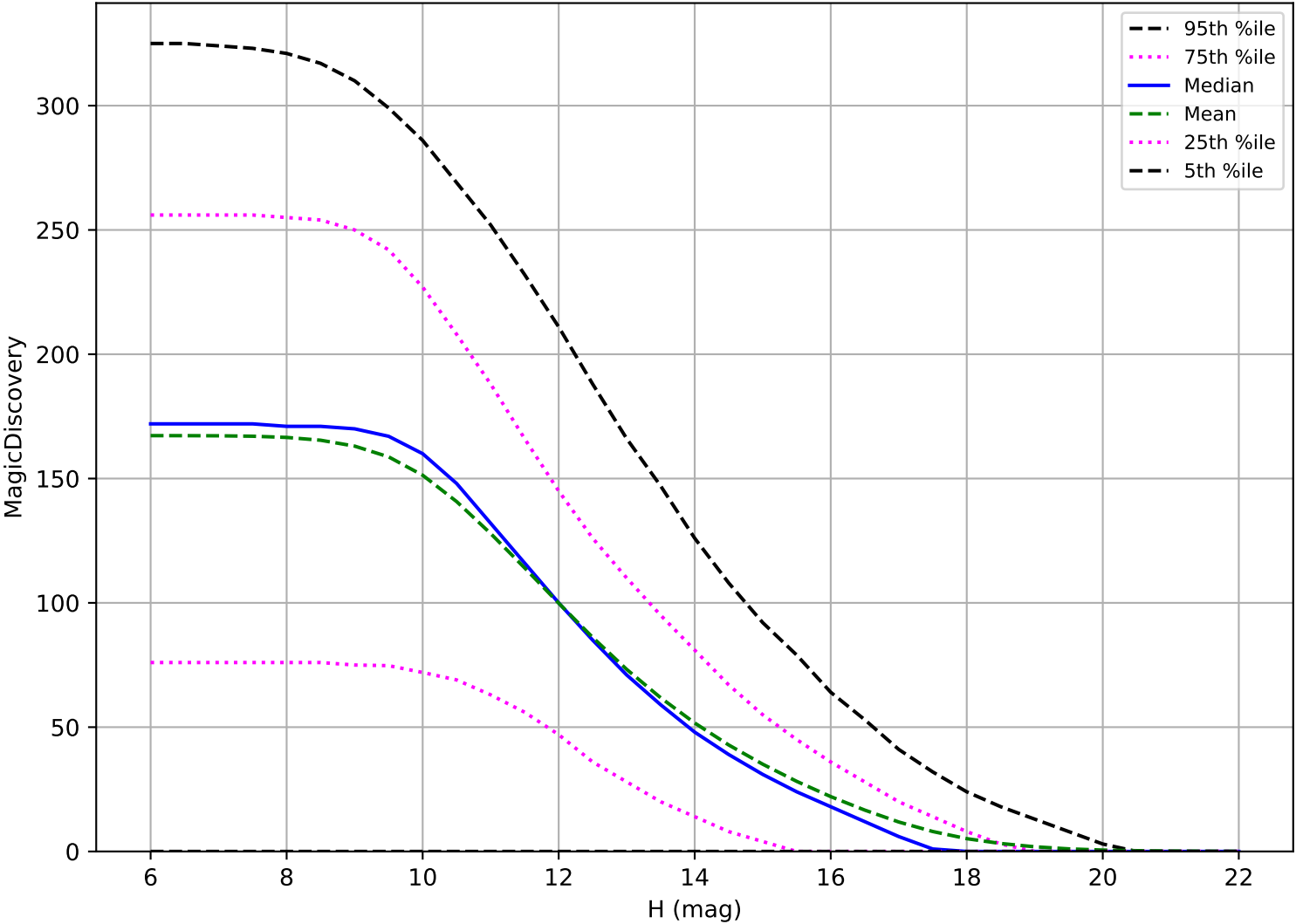
too_elab_r256_d3_ugrizy_v3.4_10yrs: OCC_r5 6 detections in 60 nights detection loss
