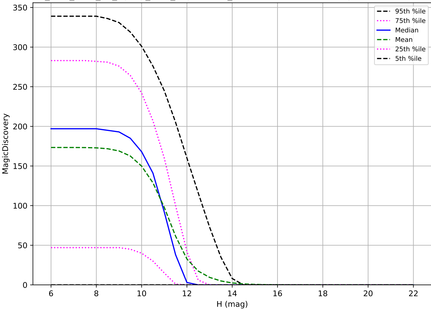
too_elab_r256_d3_ugrizy_v3.4_10yrs: OCC_r20 6 detections in 60 nights detection loss
