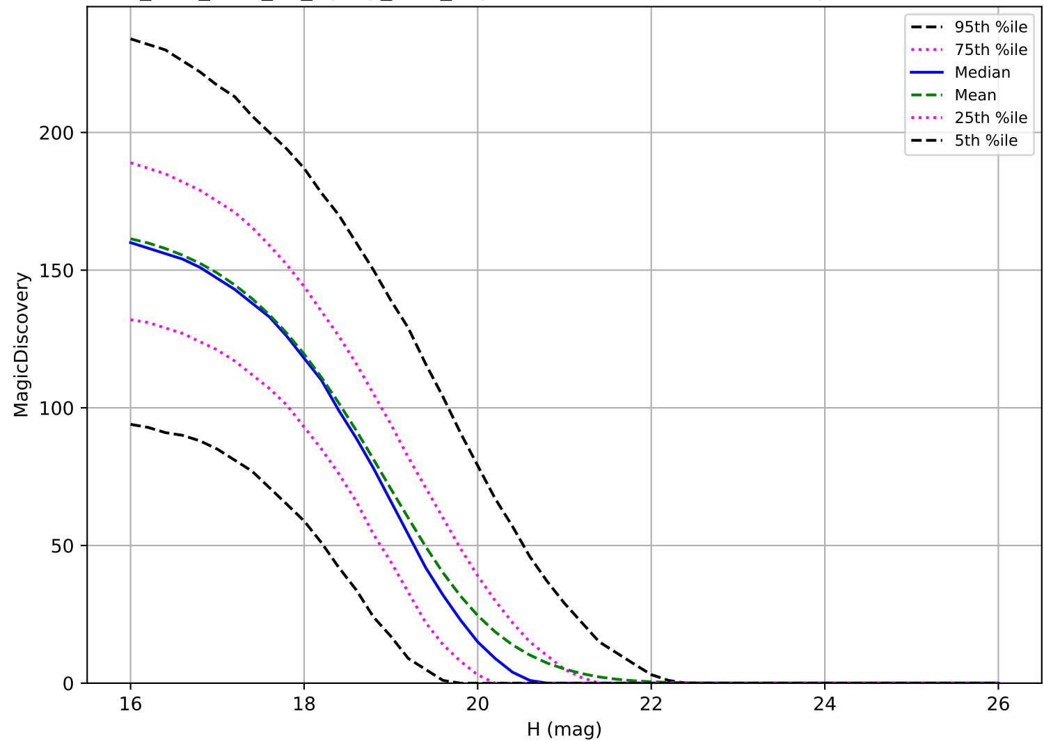
too_elab_r256_d3_ugrizy_v3.4_10yrs: MBA 6 detections in 60 nights detection loss
