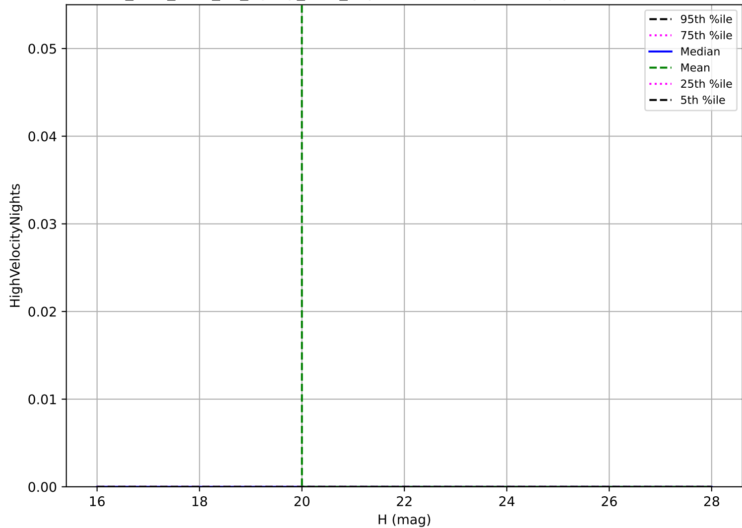
too_elab_r256_d3_ugrizy_v3.4_10yrs: Vatira High velocity pair detection loss
