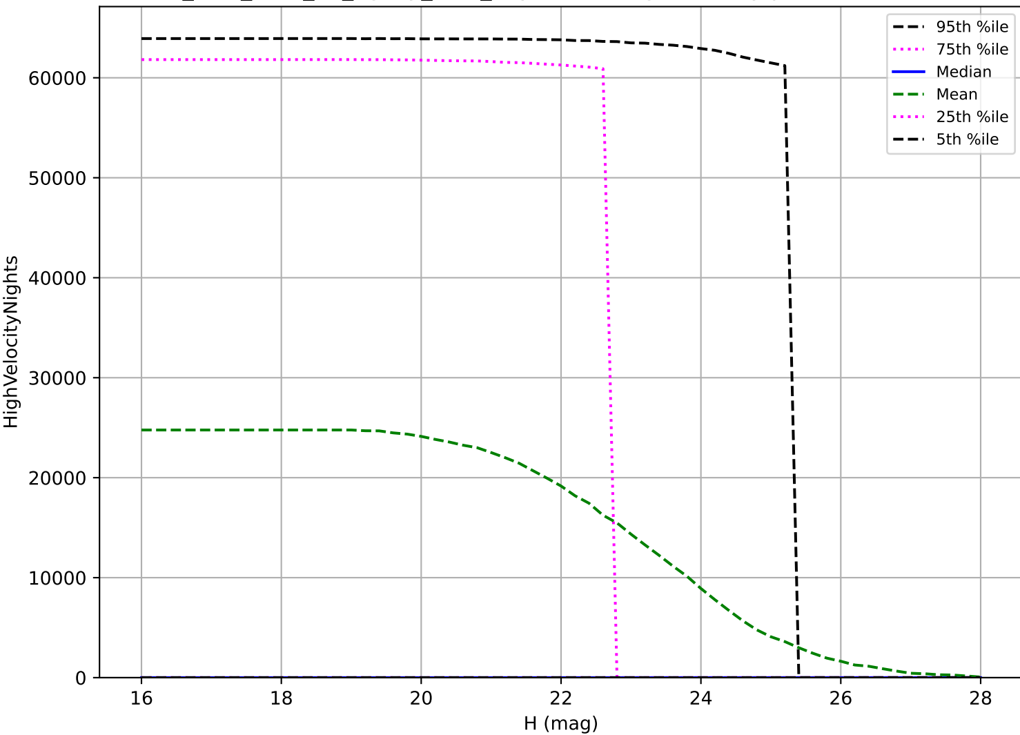
too_elab_r256_d3_ugrizy_v3.4_10yrs: PHA High velocity pair detection loss
