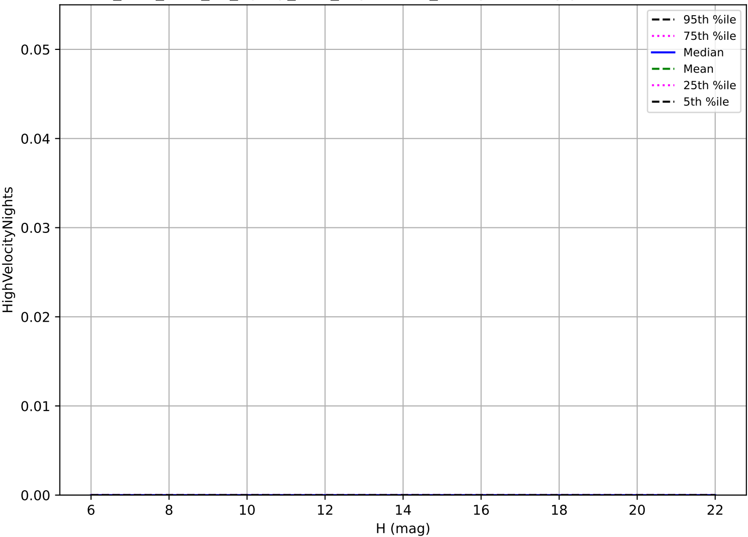
too_elab_r256_d3_ugrizy_v3.4_10yrs: OCC_r5 High velocity pair detection loss
