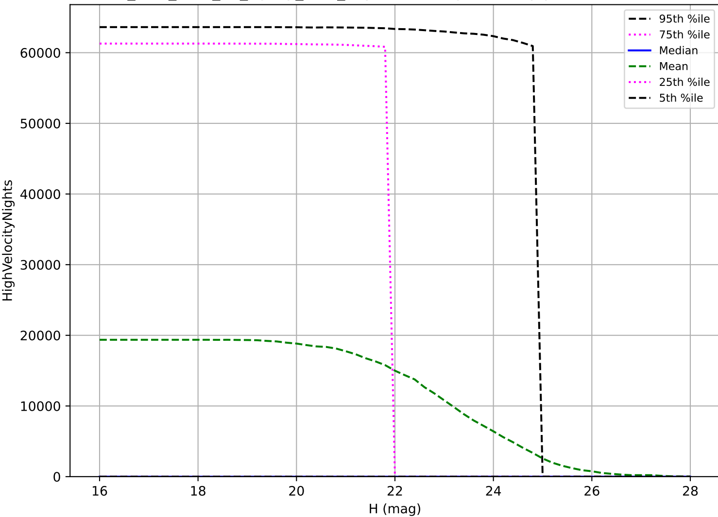
too_elab_r256_d3_ugrizy_v3.4_10yrs: NEO High velocity pair detection loss
