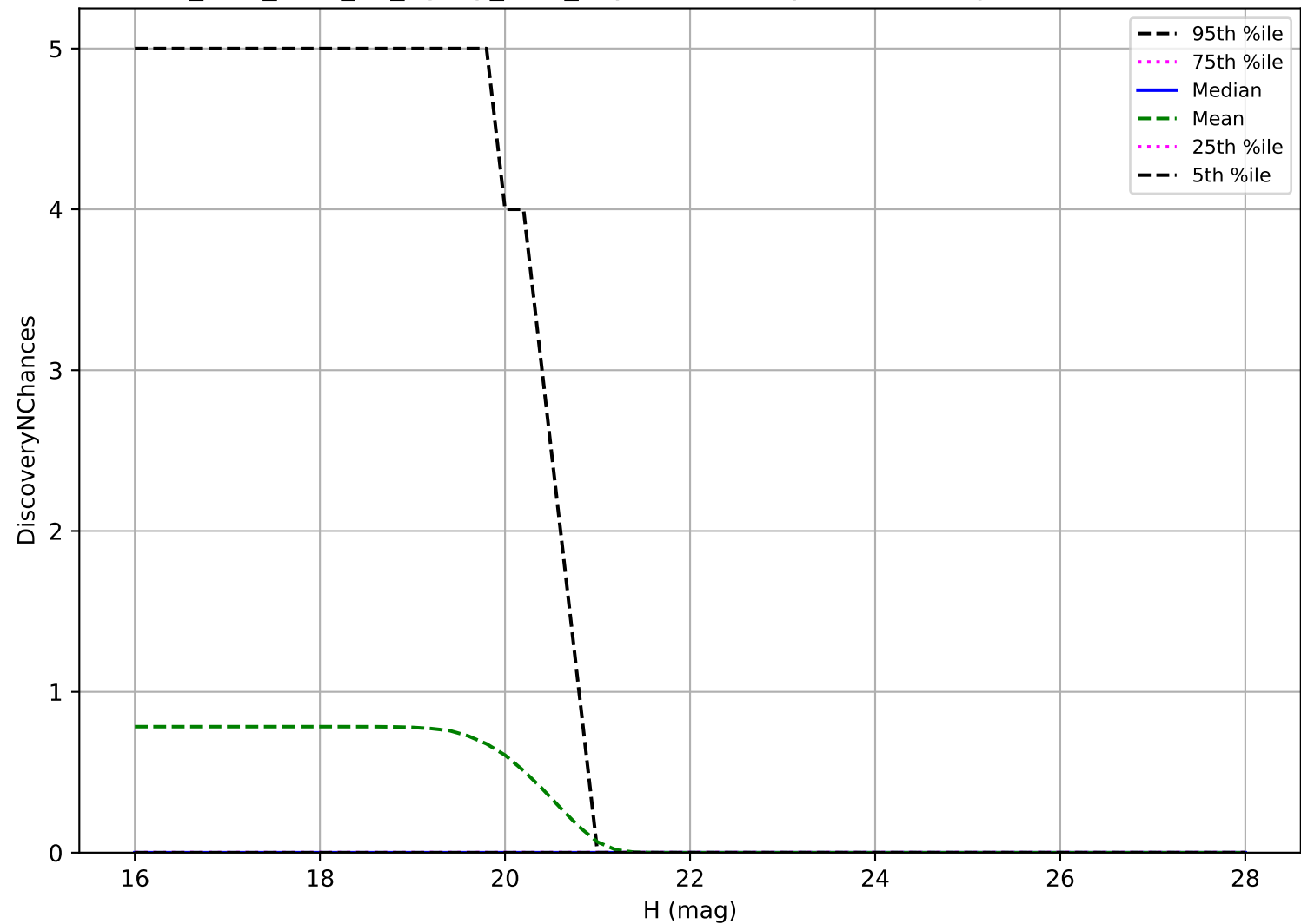
too_elab_r256_d3_ugrizy_v3.4_10yrs: Vatira 3 pairs in 15 nights detection loss
