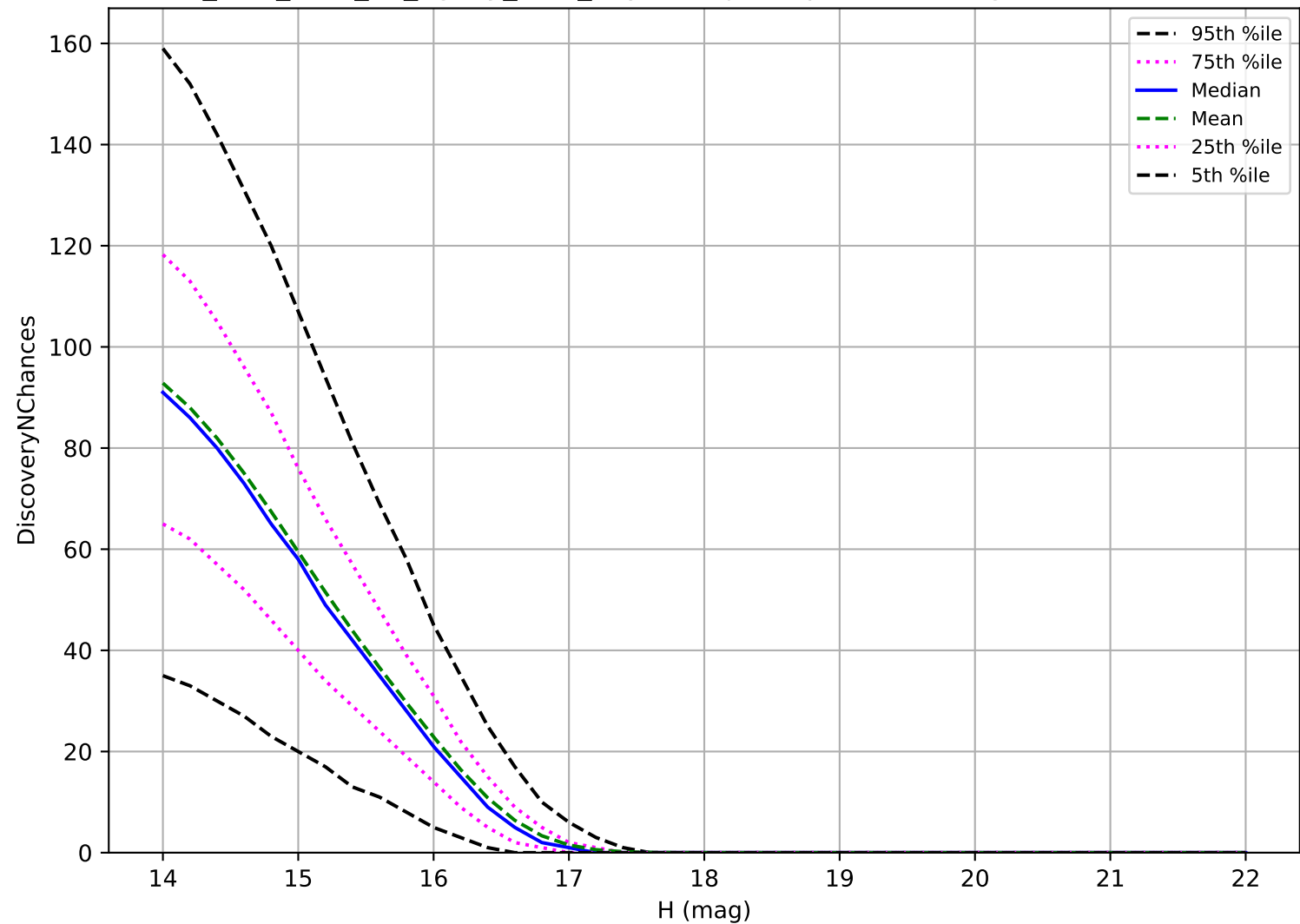
too_elab_r256_d3_ugrizy_v3.4_10yrs: Trojan 3 pairs in 15 nights detection loss
