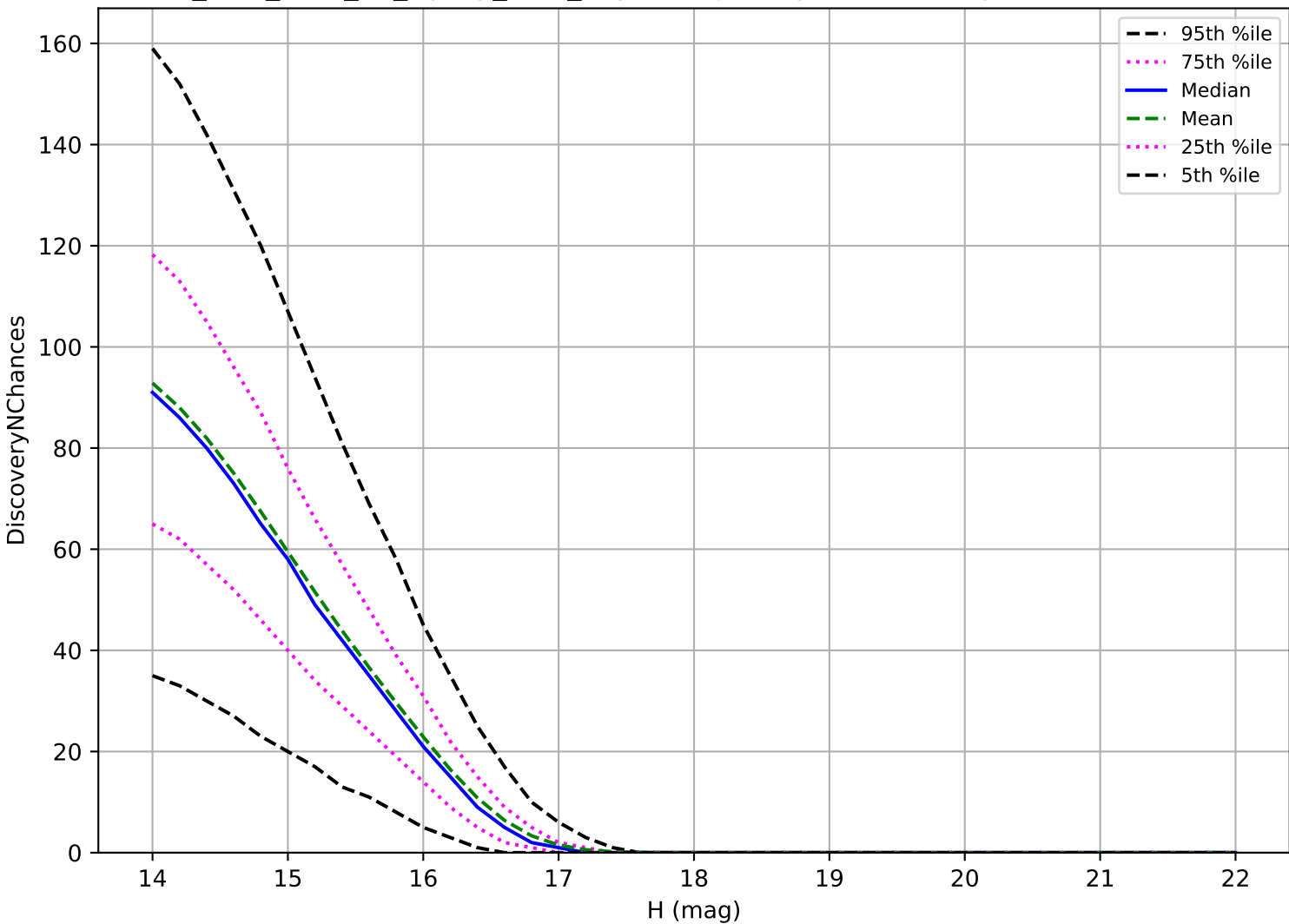
too_elab_r256_d3_ugrizy_v3.4_10yrs: Trojan 3 pairs in 15 nights detection loss
