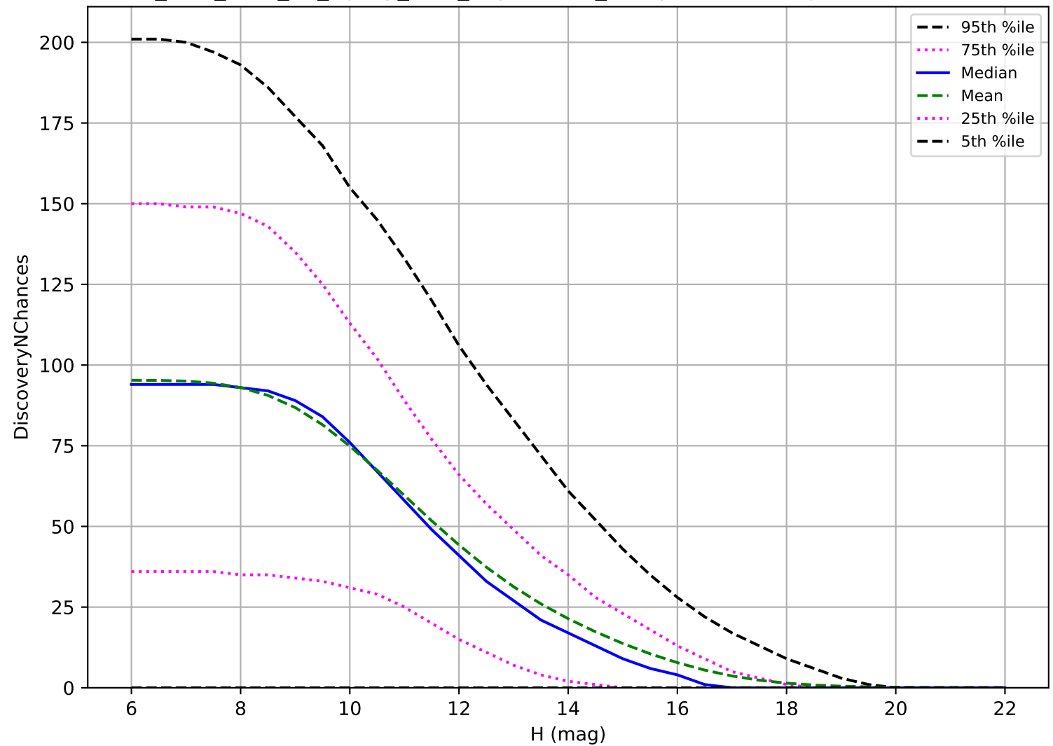
too_elab_r256_d3_ugrizy_v3.4_10yrs: OCC_r5 3 pairs in 15 nights detection loss
