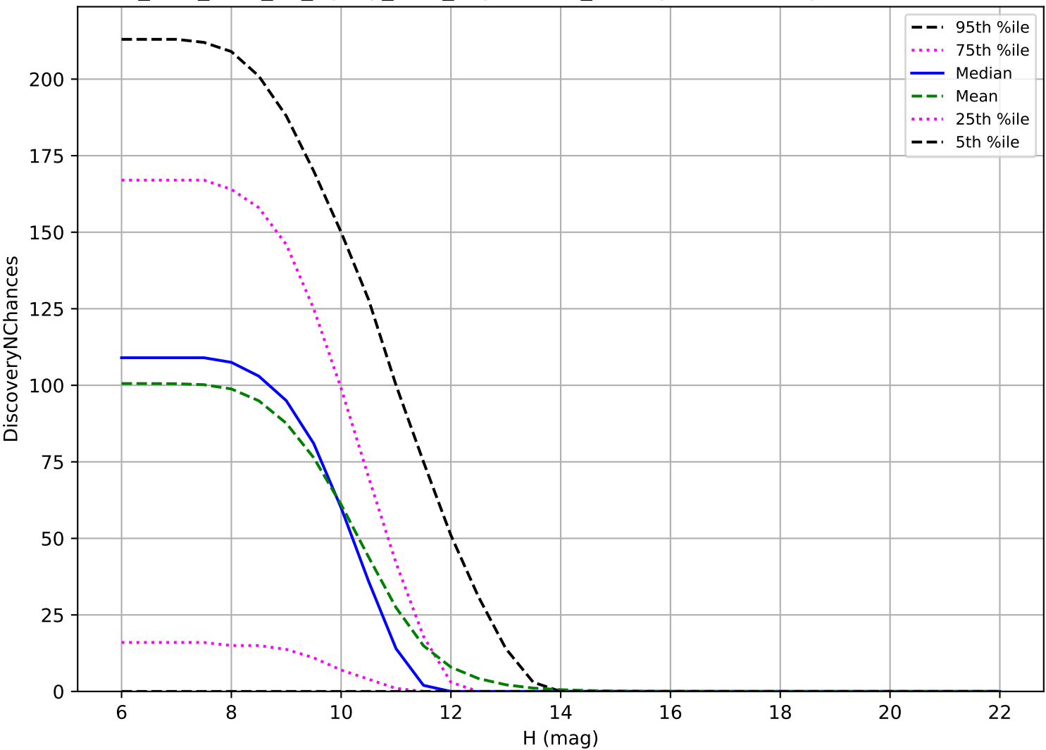
too_elab_r256_d3_ugrizy_v3.4_10yrs: OCC_r20 3 pairs in 15 nights detection loss
