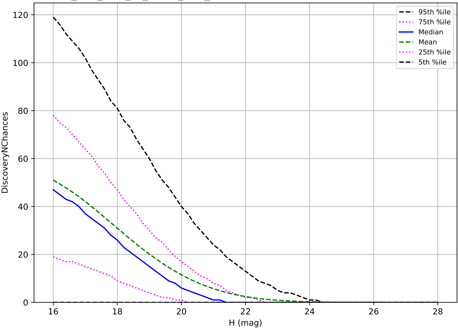
too_elab_r256_d3_ugrizy_v3.4_10yrs: NEO 3 pairs in 15 nights detection loss
