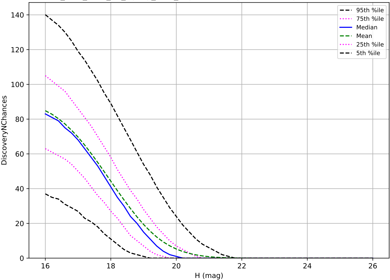
too_elab_r256_d3_ugrizy_v3.4_10yrs: MBA 3 pairs in 15 nights detection loss
