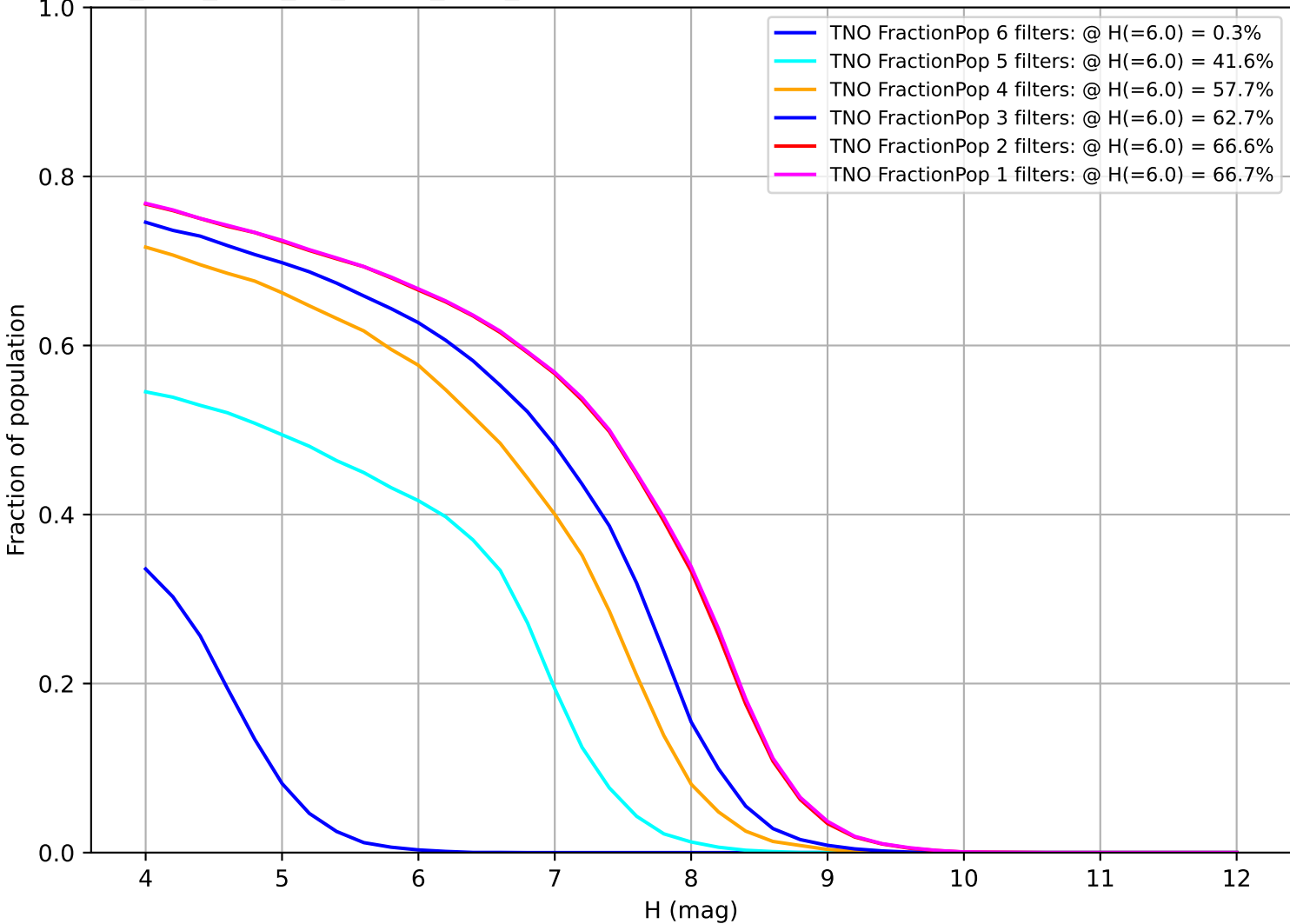
too_elab_r256_d3_ugrizy_v3.4_10yrs: Fraction of population with colors in X filters TNO
