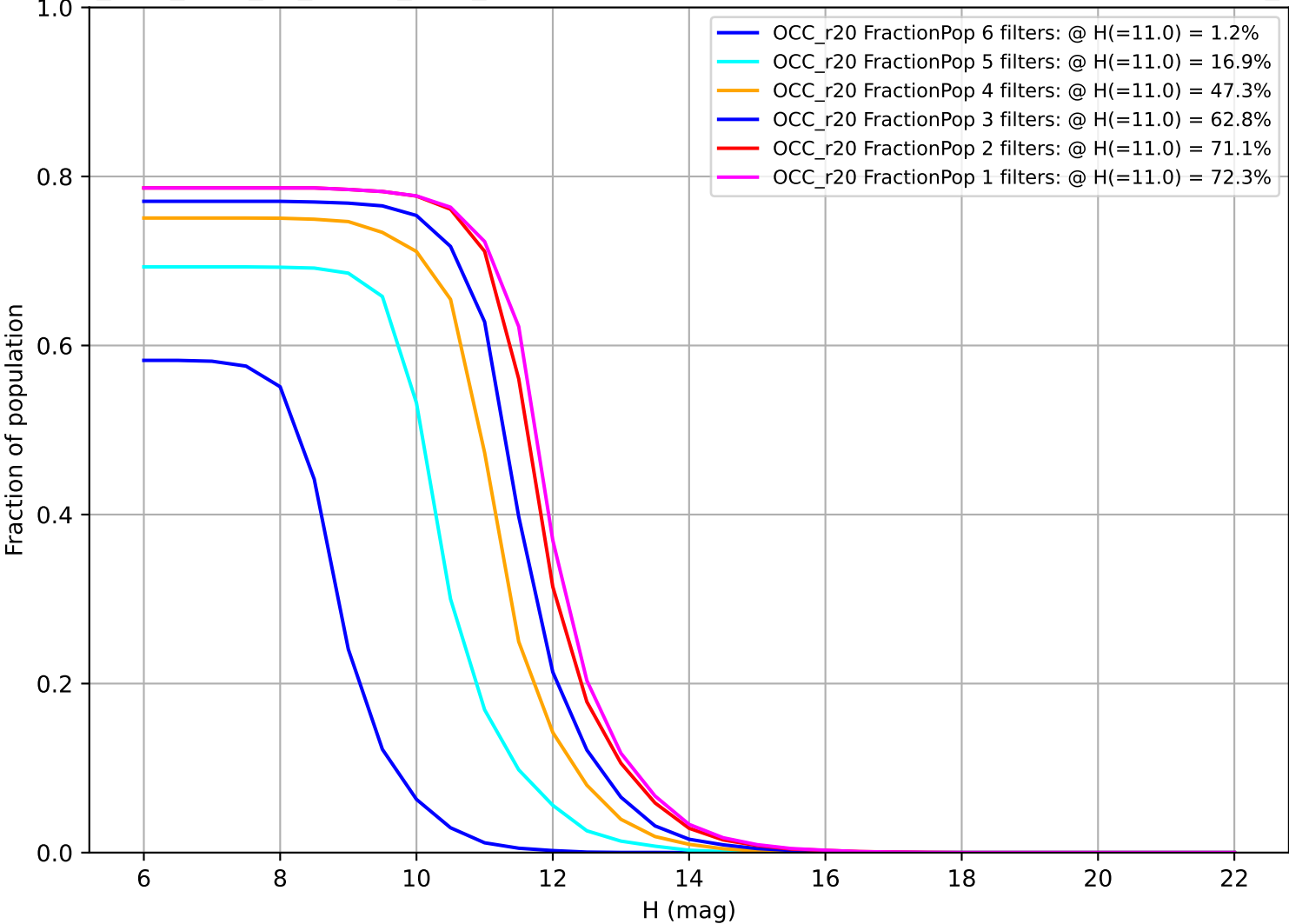
too_elab_r256_d3_ugrizy_v3.4_10yrs: Fraction of population with colors in X filters OCC_r20
