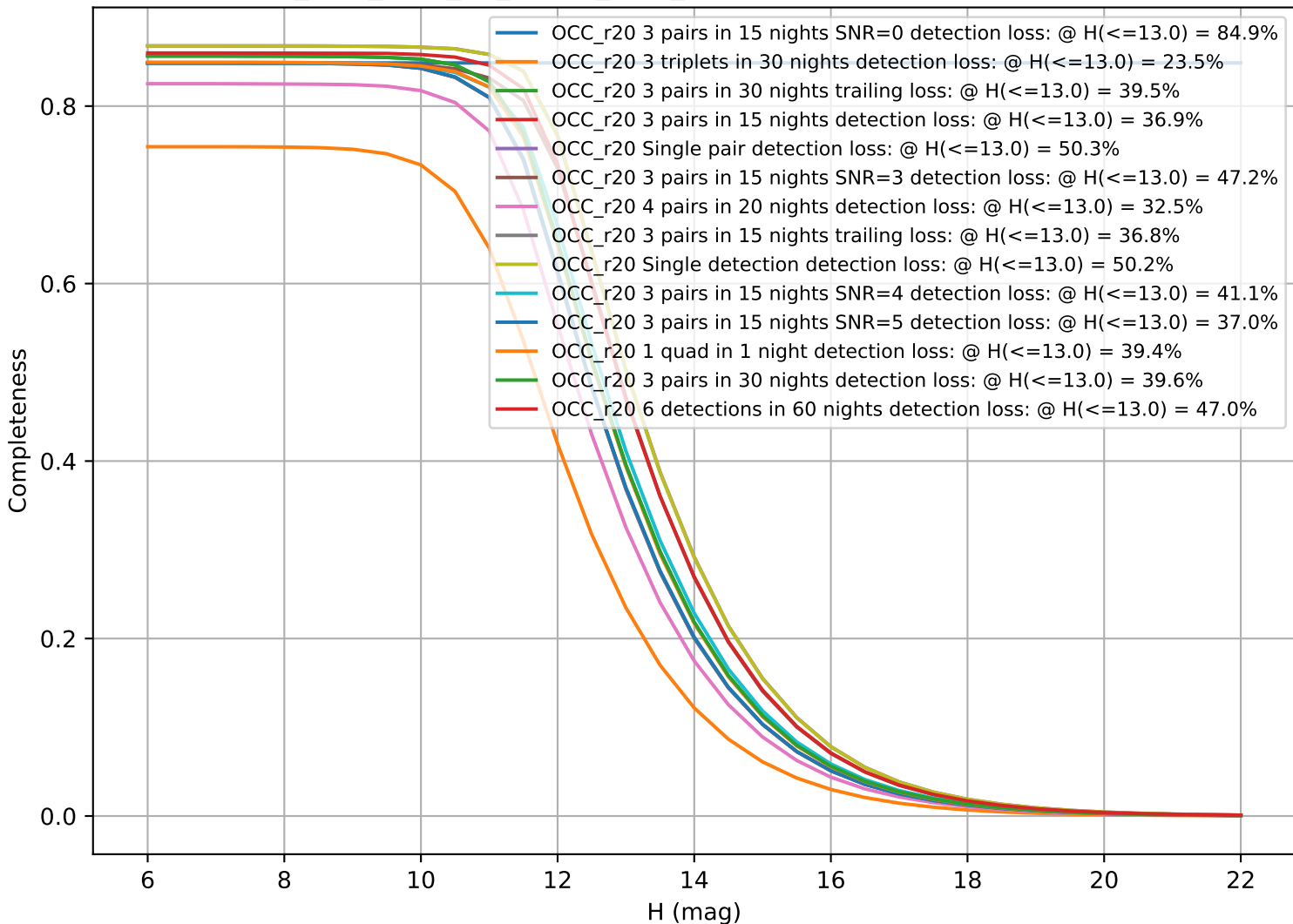
too_elab_r256_d3_ugrizy_v3.4_10yrs: CumulativeCompleteness
