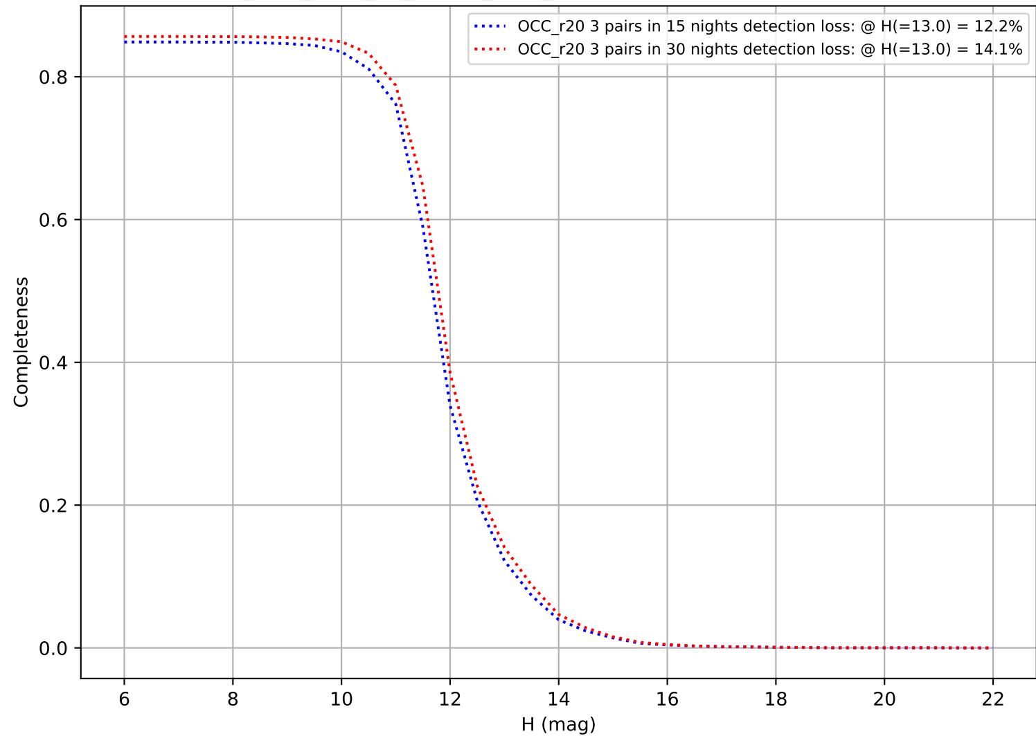
too_elab_r256_d3_ugrizy_v3.4_10yrs: DifferentialCompleteness
