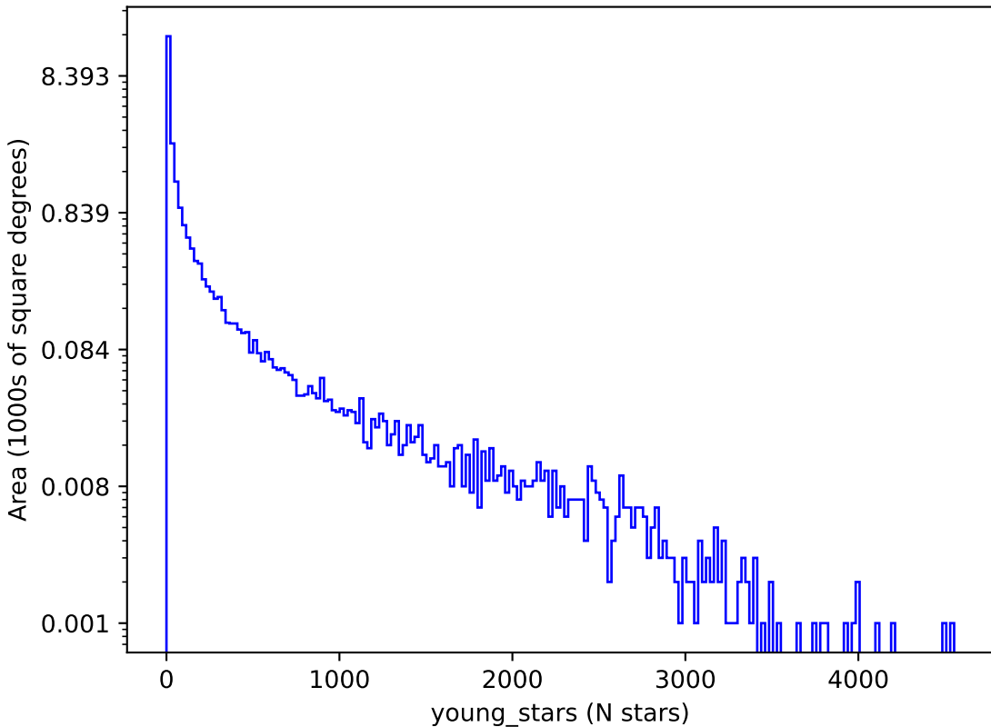
too_elab_r256_d3_ugrizy_v3.4_10yrs : young_stars
