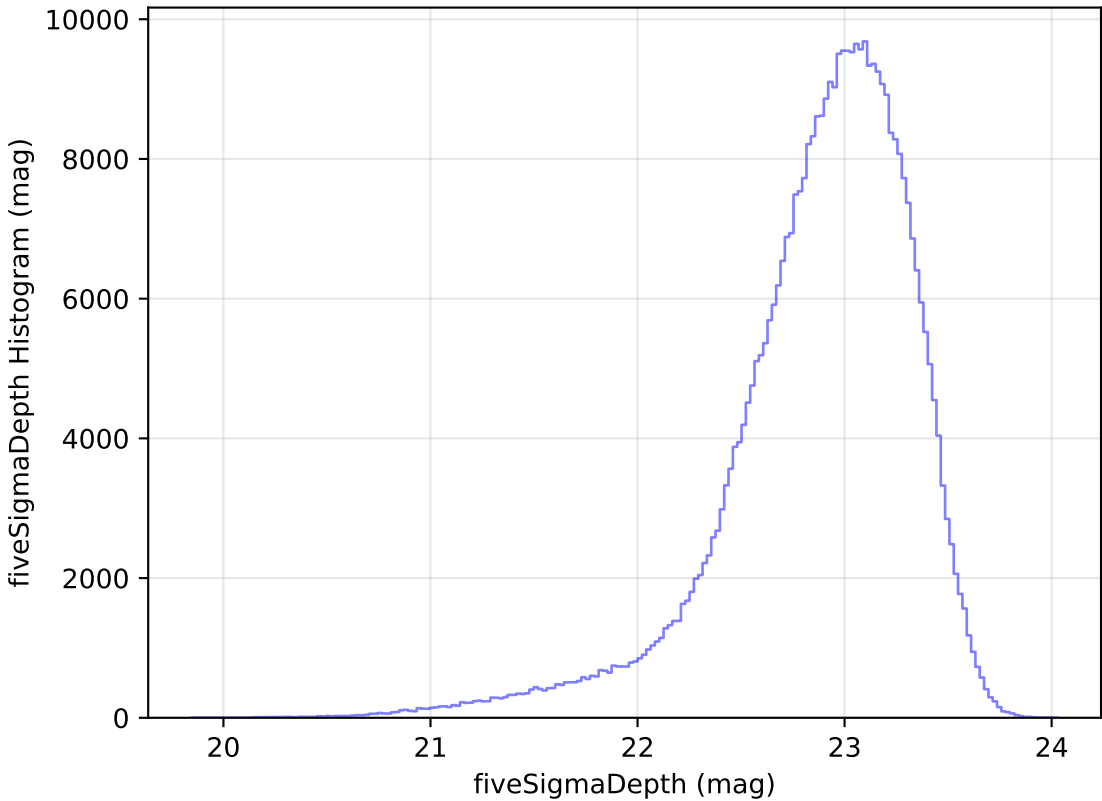
too_elab_r256_d3_ugrizy_v3.4_10yrs z: fiveSigmaDepth Histogram
