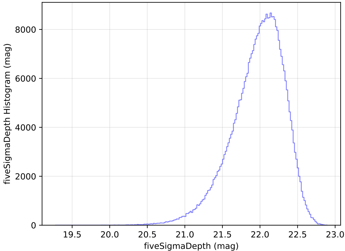
too_elab_r256_d3_ugrizy_v3.4_10yrs y: fiveSigmaDepth Histogram
