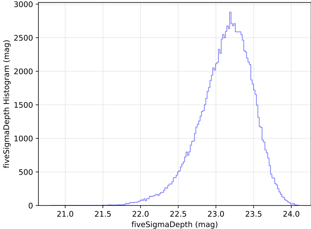
too_elab_r256_d3_ugrizy_v3.4_10yrs u: fiveSigmaDepth Histogram
