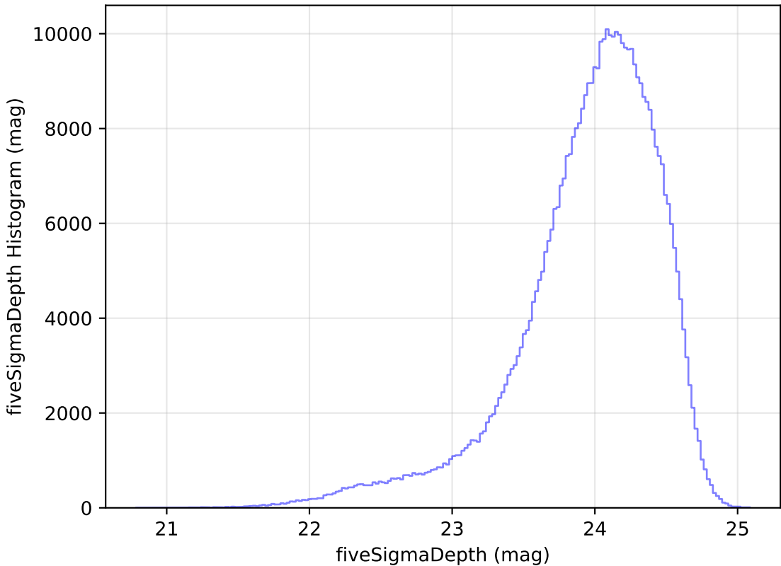
too_elab_r256_d3_ugrizy_v3.4_10yrs r: fiveSigmaDepth Histogram
