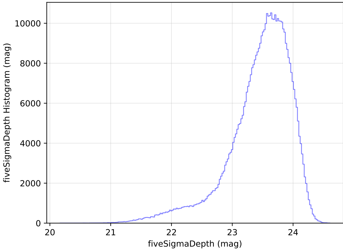
too_elab_r256_d3_ugrizy_v3.4_10yrs i: fiveSigmaDepth Histogram
