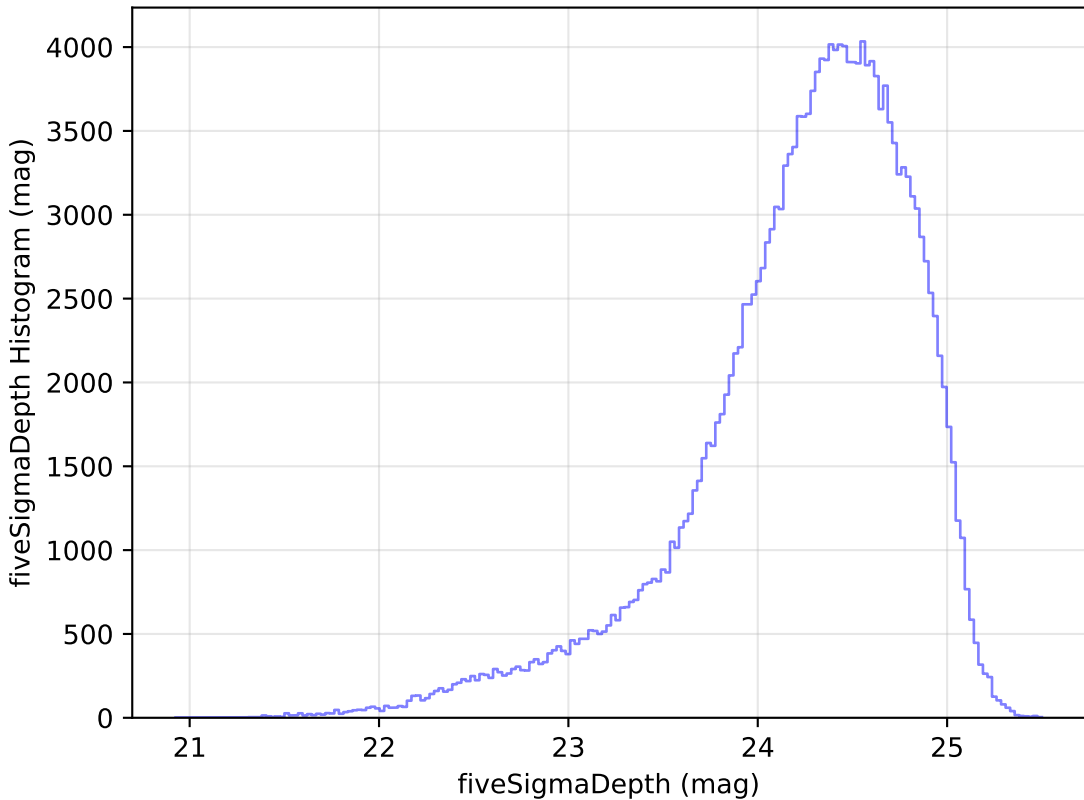
too_elab_r256_d3_ugrizy_v3.4_10yrs g: fiveSigmaDepth Histogram
