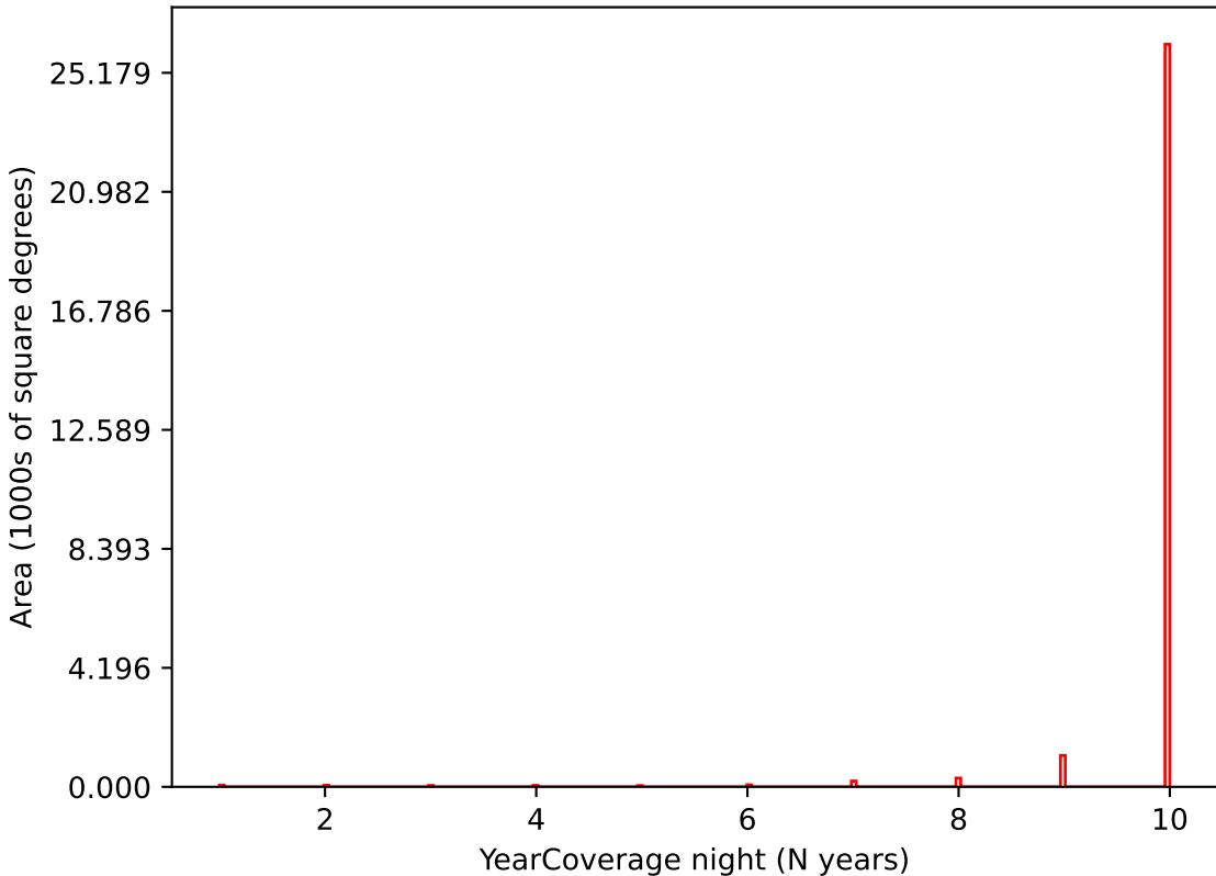
too_elab_r256_d3_ugrizy_v3.4_10yrs i band: YearCoverage night
