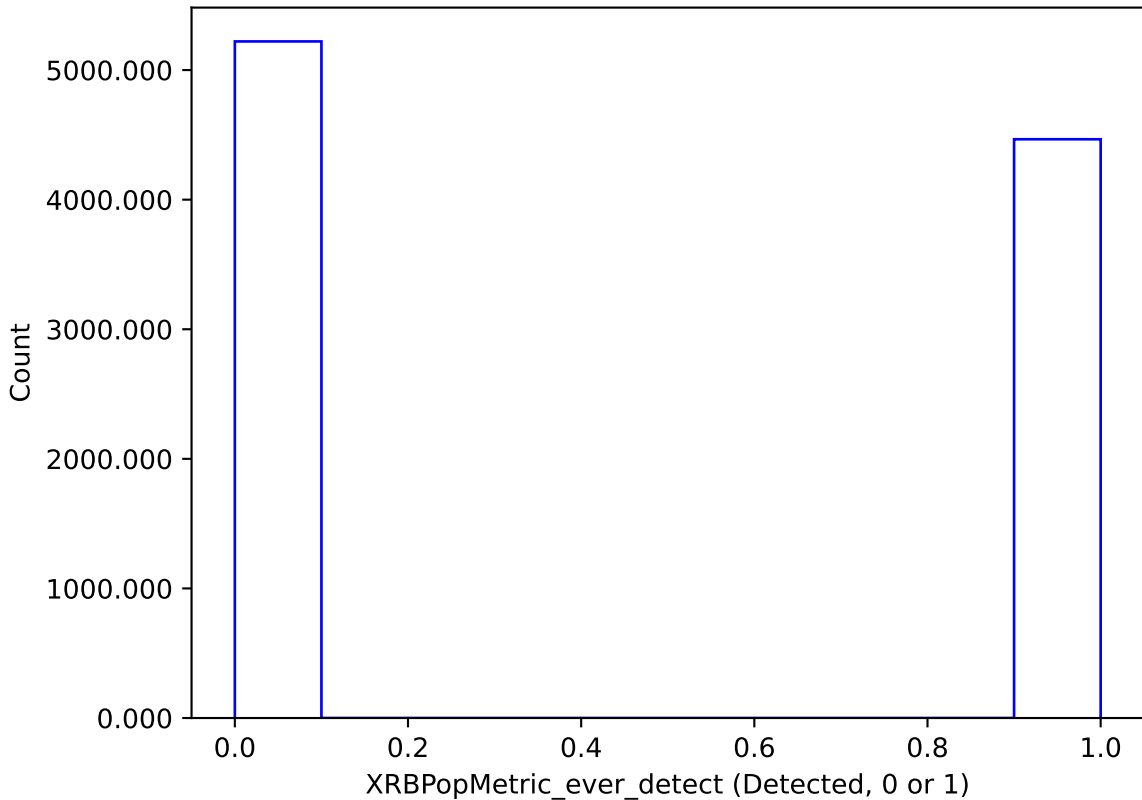
too_elab_r256_d3_ugrizy_v3.4_10yrs : XRBPopMetric_ever_detect
