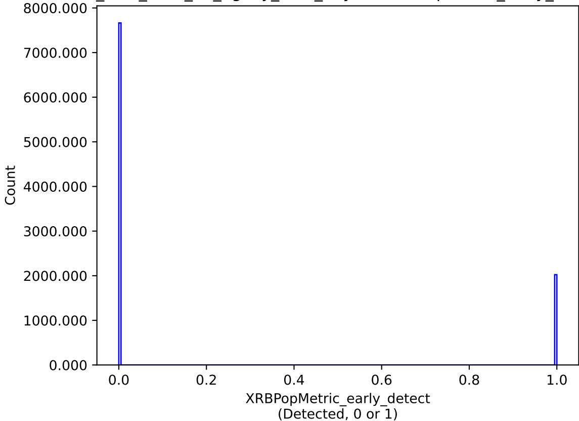
too_elab_r256_d3_ugrizy_v3.4_10yrs : XRBPopMetric_early_detect
