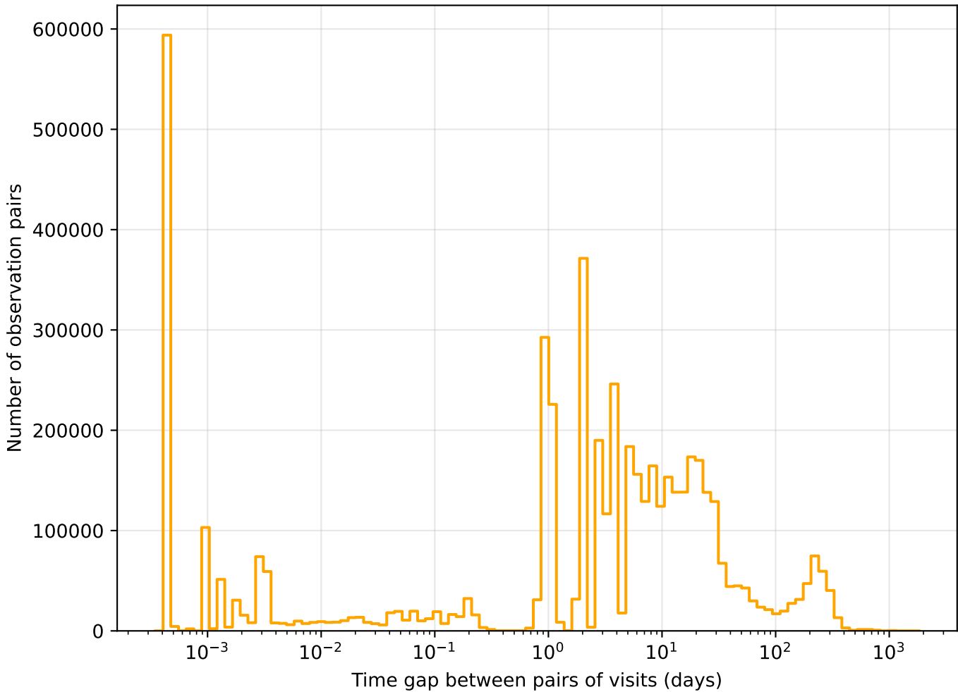
too_elab_r256_d3_ugrizy_v3.4_10yrs r band: Tgaps observationStartMJD
