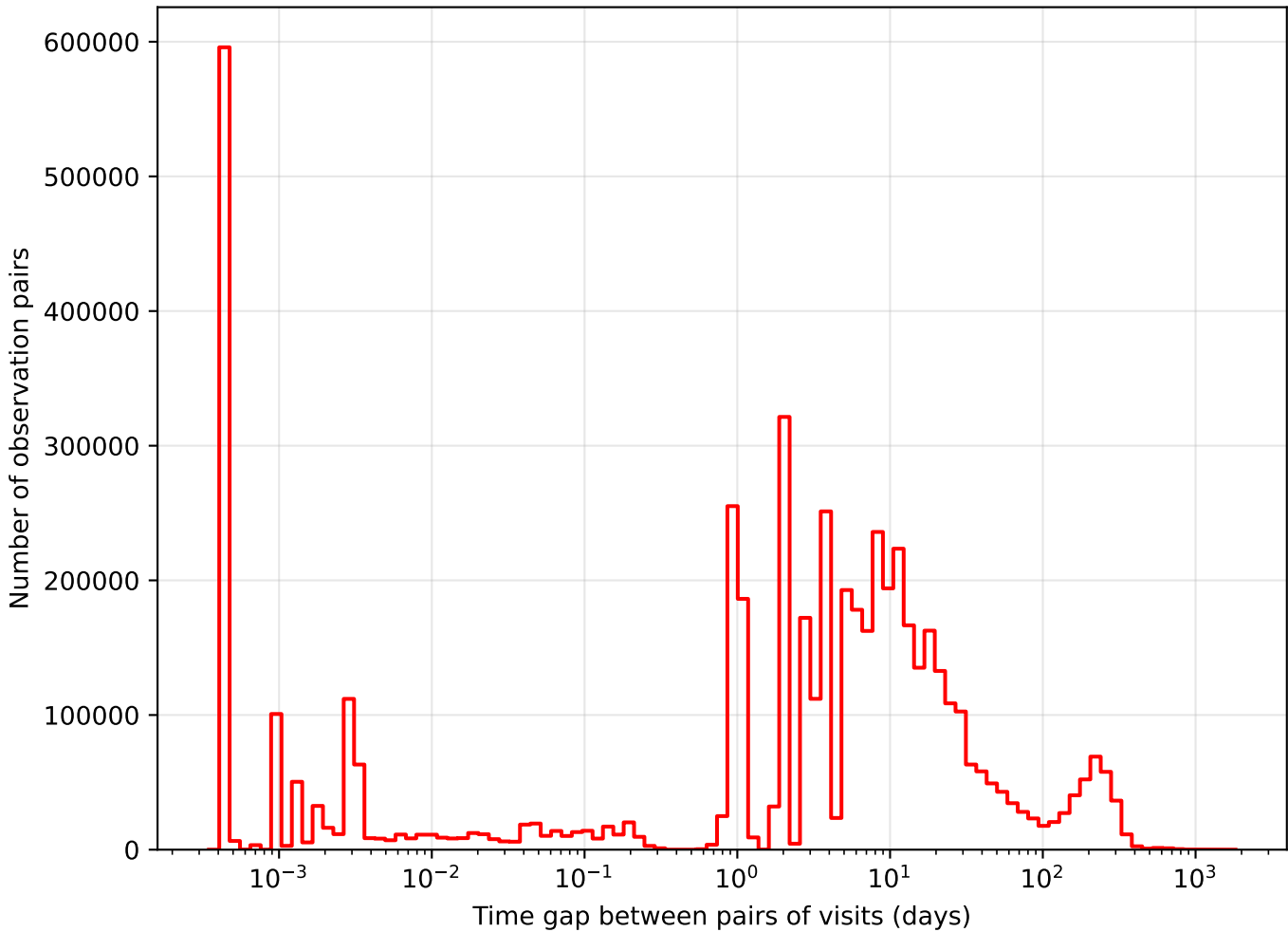
too_elab_r256_d3_ugrizy_v3.4_10yrs i band: Tgaps observationStartMJD
