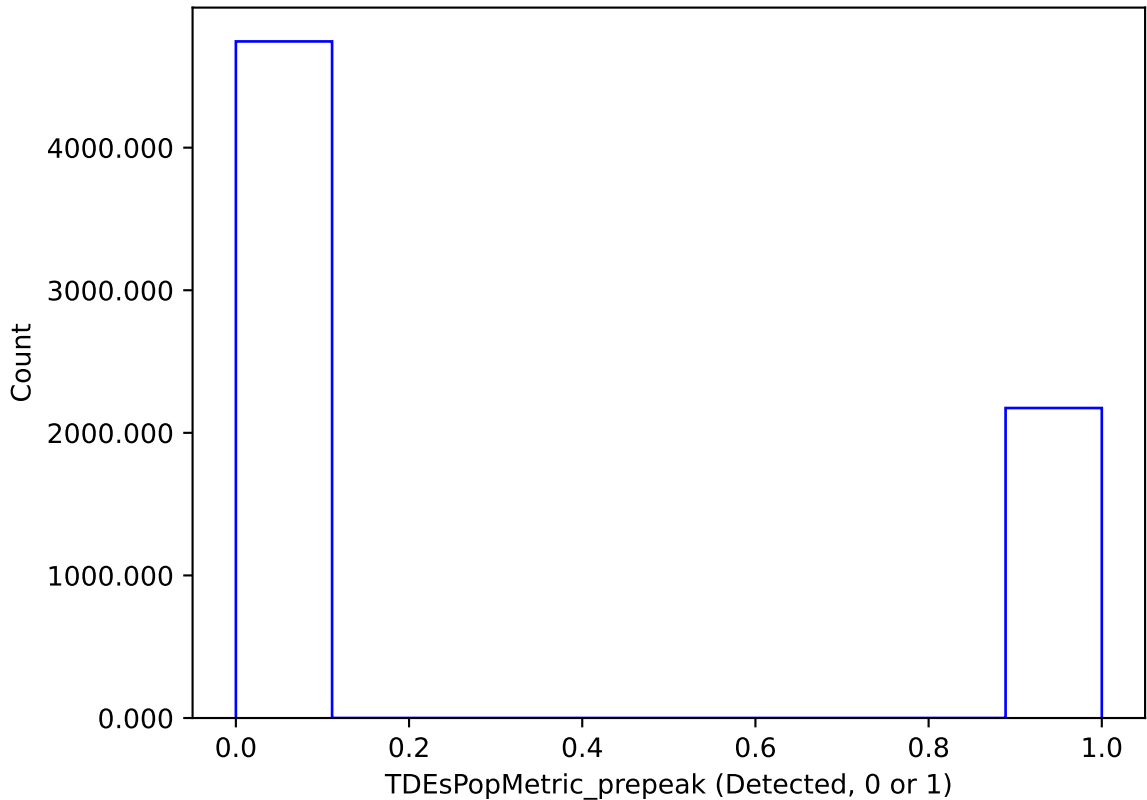
too_elab_r256_d3_ugrizy_v3.4_10yrs : TDEsPopMetric_prepeak
