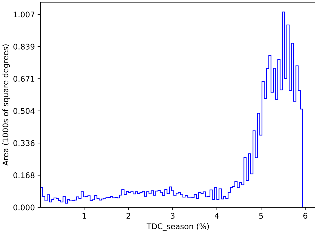
too_elab_r256_d3_ugrizy_v3.4_10yrs : TDC_season
