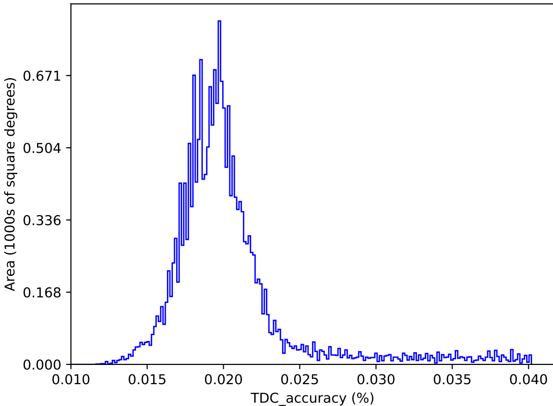
too_elab_r256_d3_ugrizy_v3.4_10yrs : TDC_accuracy
