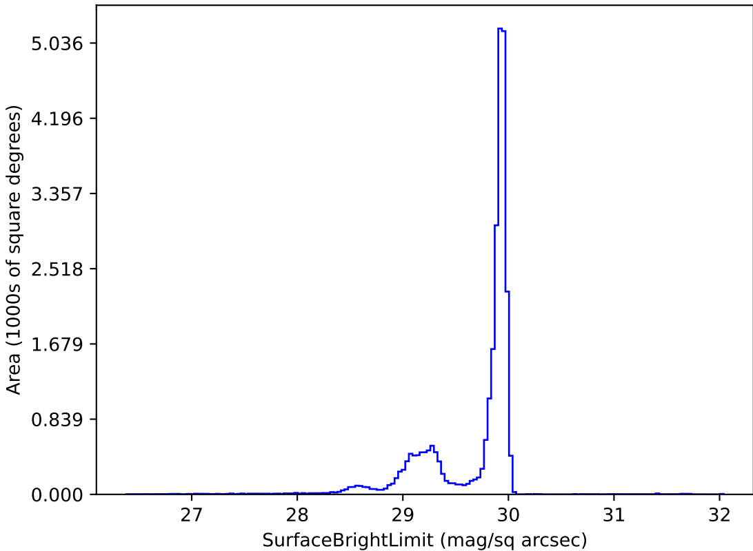
too_elab_r256_d3_ugrizy_v3.4_10yrs i: SurfaceBrightLimit
