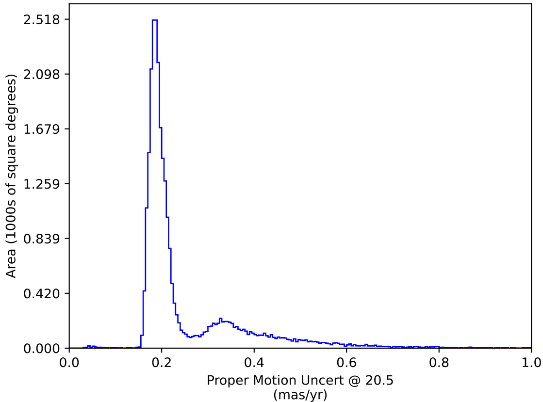
too_elab_r256_d3_ugrizy_v3.4_10yrs : Proper Motion Uncert @ 20.5
