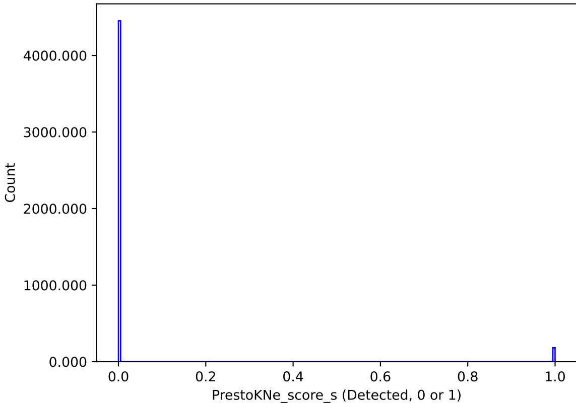
too_elab_r256_d3_ugrizy_v3.4_10yrs : PrestoKNe_score_s
