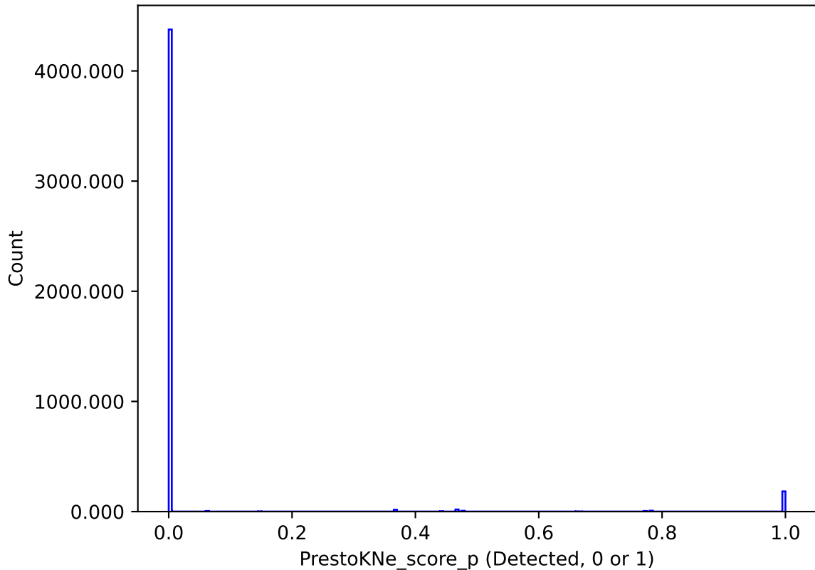
too_elab_r256_d3_ugrizy_v3.4_10yrs : PrestoKNe_score_p
