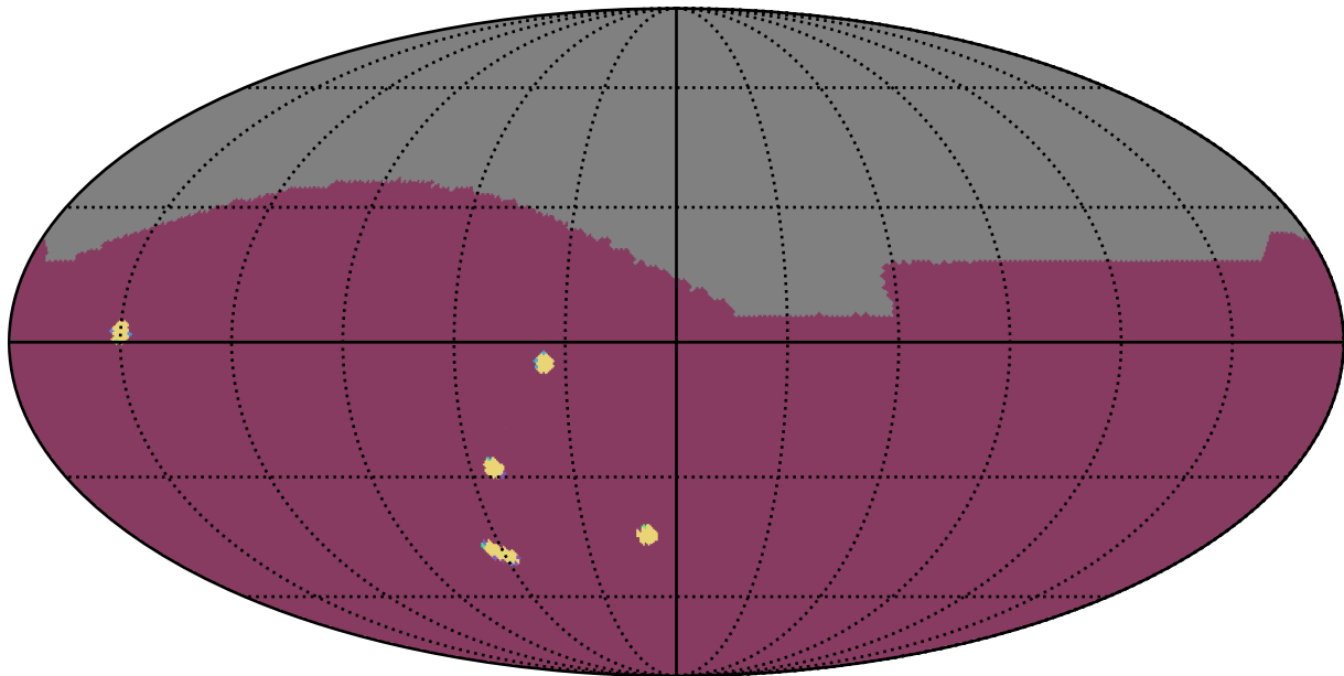
too_elab_r256_d3_ugrizy_v3.4_10yrs : NumberOfQuickRevisits
