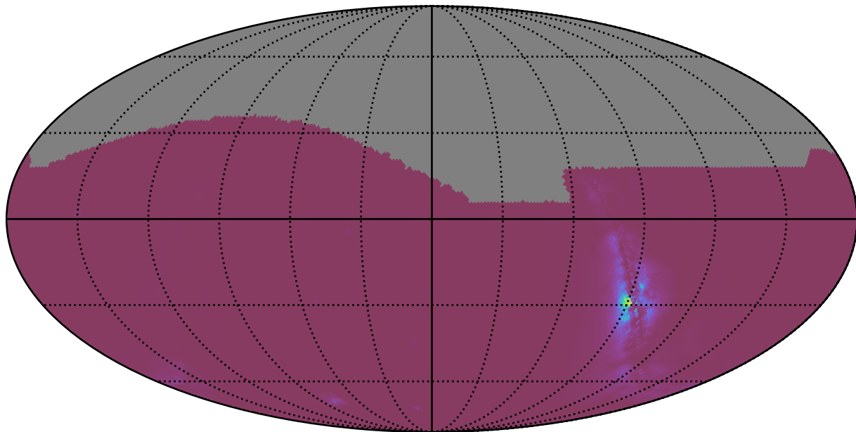
too_elab_r256_d3_ugrizy_v3.4_10yrs : NlcPoints
